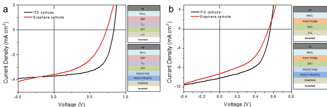
Figure 6 | J - V characteristics of representative graphene and ITO devices with ZnO ESL. Using (a) small molecule photoactive layers and (b) P3HT:PCBM photoactive layer under AM 1.5 G at 100 \text{ mW} \cdot \text{cm}^{-2} .
