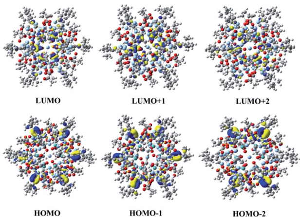
Fig. 5 The frontier molecular orbitals including HOMO–2, HOMO–1, HOMO, LUMO, LUMO+1 and LUMO+2 of the [\text{Ag}_{55}(\text{MoO}_4)_6(\text{C}\equiv\text{CtBu})_{24}(\text{CH}_3\text{COO})_{18}]^+ cluster skeleton in the \{\text{Ag}_{55}\text{Mo}_6\} nanocluster.
