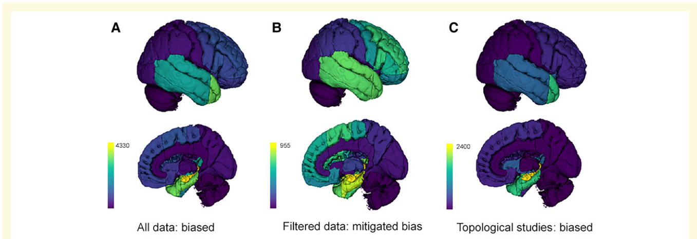
Figure 2 Database overview and publication bias. Semio2Brain Database overview. (A–C) Pseudo-glyph representations of integrated seizure semiology lateralizing and localizing values with data points (colour bars) obtained from querying the entire database (A); or querying non-topological studies only (B); or querying only data from topological studies where patients were preselected based on prior knowledge of their epileptogenic and seizure-onset zones (C). Top row: lateral views of the right hemisphere. Lower row: medial right hemispheres. These cortical heatmaps were obtained by querying the database for all semiologies. Colour bar represents number of data points.
