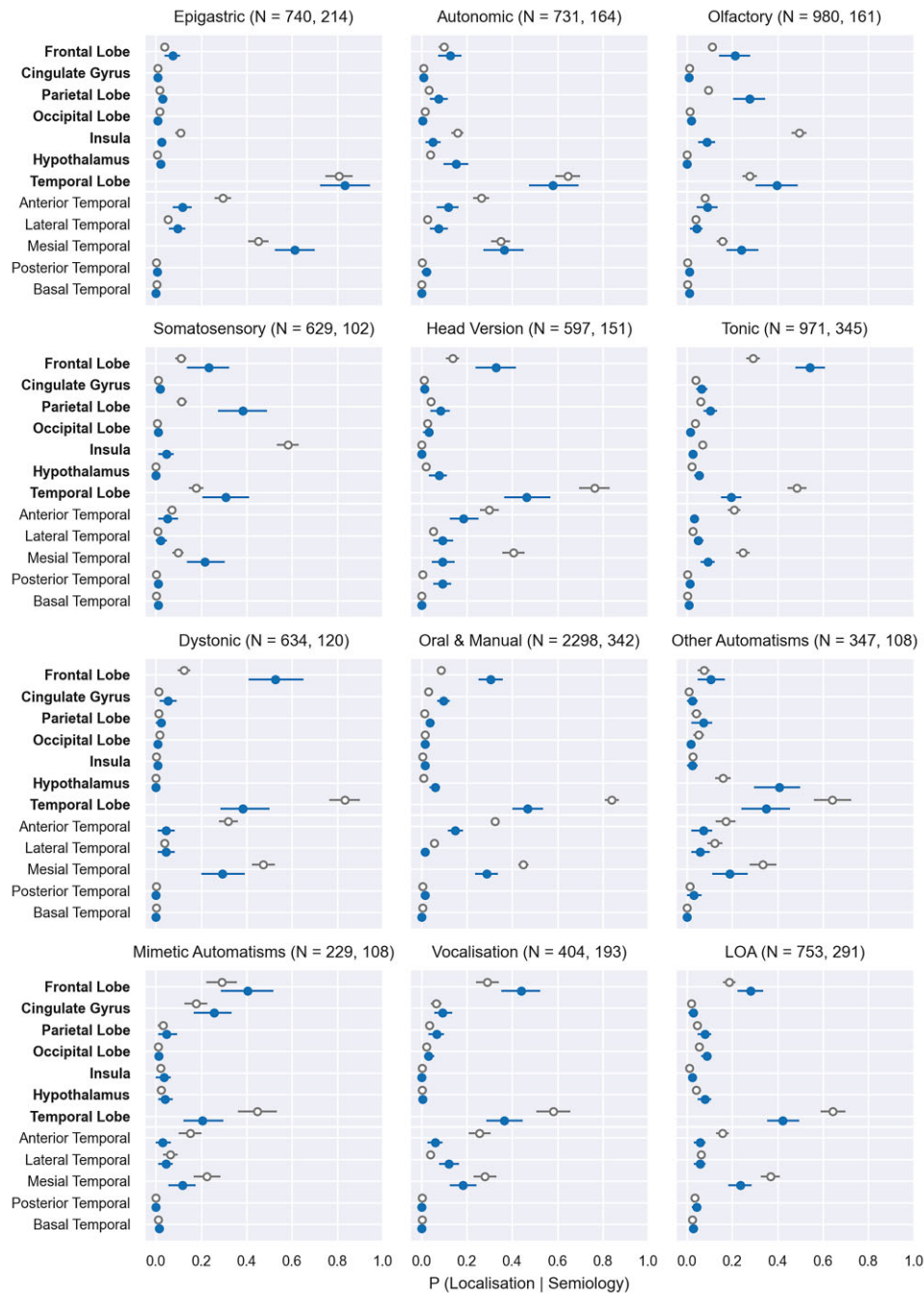
Figure 3 Forest plots. Seizure semiology localizing values for the 12 most commonly occurring semiologies: seven top-level brain regions are shown, and the temporal lobe is split into five subregions. The temporal lobe includes data points from its subregions as well undifferentiated localizations to the temporal lobe. Results from all data are in grey (empty circles) and spontaneous semiologies (non-topological studies) in blue (filled circles). Error bars represent 95% CI for 10 000 repeated bootstrapped samples. N, number of semiological data points (all data, non-topological subset). Data points are normalized to numbers of patients. LOA, loss of awareness. Oral and manual, orofacial automatisms and/or manual automotor signs.
