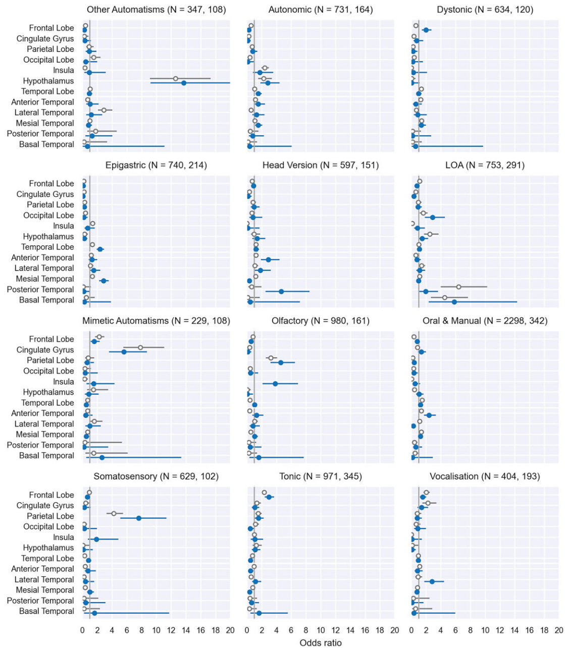
Figure 4 Relative localizing values of semiologies: Odds ratios of localizing value, given a semiology, for the 12 most commonly occurring semiologies in Semio2Brain database. These were calculated using two-by-two contingency tables from querying the entire Semio2Brain database for ictal semiologies. Blue (filled circles): spontaneous semiology (non-topological) data points. Grey (empty circles): all data.
