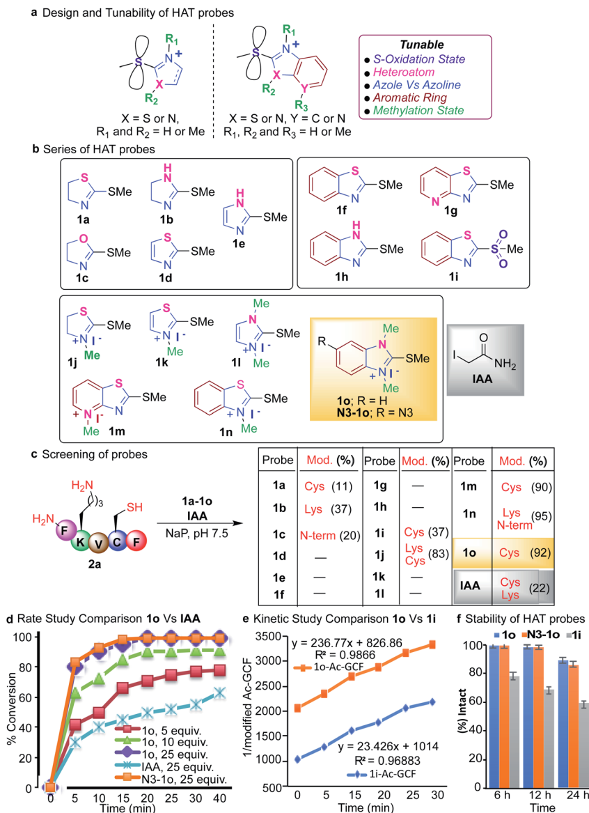
Fig. 2 Tunable and stable HAT probes for targeting cysteine. (a) Design of hydrolytically stable thioether probes to tune their reactivity and selectivity for modification of cysteine. (b) Structures of a variety of HAT probes with different modifications to investigate their reactivity and selectivity for cysteine. (c) Screening of probes (40 mM, 10 equiv.) by using peptide FKVCF (4 mM, 1 equiv.) with all the nucleophilic residues and comparison with well known IAA and sulfone probe (1i) (40 mM) under physiological conditions (NaP (10 mM), pH 7.5, 25 °C) for 3 h. Probe 1o showed high selectivity and reactivity for cysteine as compared to sulfone probe 1i and IAA. (d) Observed rate of the modification of cysteine of the peptide Ac-GCF 2b (0.003 mM) with 1o (5–25 equiv.), its azide analog N3-1o (0.6 mM, 25 equiv.) and IAA (0.6 mM, 25 equiv.) in 10 mM phosphate buffer (pH 7.5, 25 °C) at different time intervals. (e) Kinetics study comparison of probe 1o (0.973 mM) and 1i for labelling peptide Ac-GCF 2b (0.973 mM) showed a 10 fold faster rate of probe 1o for cysteine modification as compared to sulfone analog 1i (0.973 mM) under physiological conditions (NaP (10 mM), pH 7.5, 25 °C). In both (d) and (e), each time point represents an average of three independent experiments. (f) High stability of probe 1o (38.75 mM) and its azide analog N3-1o (38.75 mM) as compared to sulfone probe 1i (38.75 mM) under physiological conditions (NaP (10 mM), pH 7.5, 25 °C).
