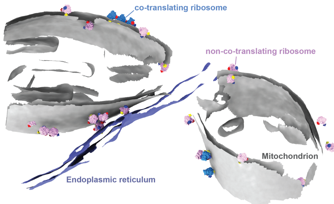
Supplementary Figure 6. Cytoplasmic ribosomes primed for protein import cluster on the mitochondrial membrane.
