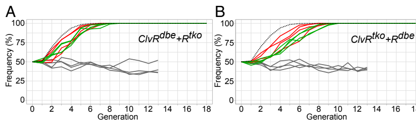
Fig. 4. ClvR n+1 + R n selfish elements drive into populations carrying ClvR n . Shown are the drive outcomes for ClvR dbe + R tko driving into a population of w 1118 (red lines), ClvR tko (green lines), and ClvR dbe (gray lines, control) (A), and ClvR tko + R dbe driving into a population of w 1118 (red lines), ClvR dbe (green lines), and ClvR tko (gray lines, control) (B). There are four replicates for each drive experiment. Dashed black lines represent model estimated behavior for the spread of ClvR n+1 with no fitness cost into populations consisting primarily of ClvR n population (see Methods for model details). Allele frequencies at generation 12 are presented in SI Appendix, Tables S11 and S12 .
