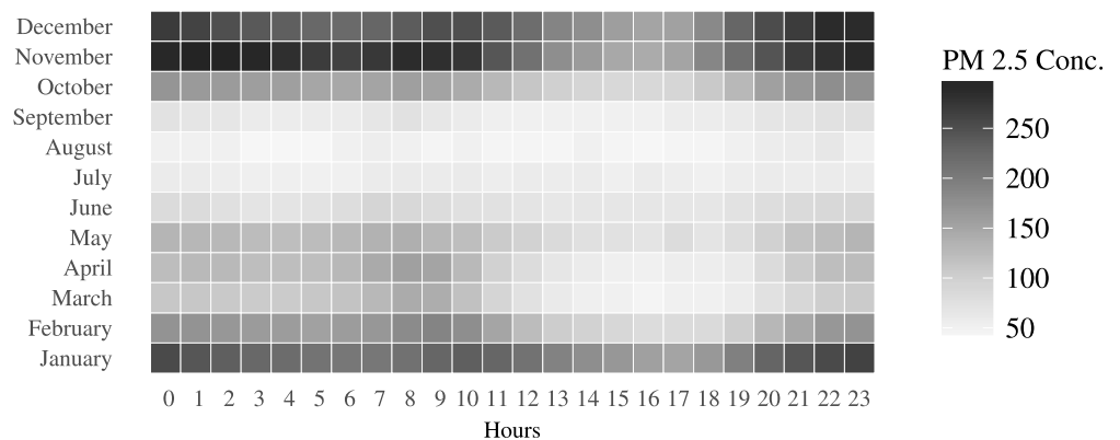
Fig 3. Location effect in pollution levels.
