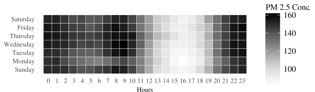
Fig 1. Week effect in pollution levels.
