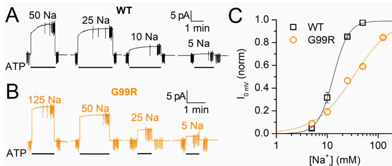
Figure 10. Na + o dependence of wild-type and G99R pumps. (A and B) Representative current recordings at 0 mV from giant inside-out patches excised from an oocyte expressing wild type (A) or one expressing G99R (B). The patches were perfused with intracellular solutions of varying [Na + i ] (a mix of Na + i and K + i solutions; Materials and methods). Application of 4 mM ATP, induced outward pump currents in a [Na + i ]-dependent manner. Vertical deflections represent 25-ms voltage steps. (C) Mean [Na + i ]-dependence of ATP-induced currents normalized to the I_{max} from Hill fits to the mean data for wild type (squares, n = 5 ) and G99R (circles, n = 4 ) with parameters K_{0.5} = 13.1 mM, n_H = 2.9 for wild type and K_{0.5} = 33.1 mM, n_H = 1.2 for G99R (mean from fits in individual experiments are shown in the text). Mean ATP-induced current was 12.4 \pm 2.6 pA in 50 mM Na + i 90 mM K + i for wild type and 12.4 \pm 1.3 pA in 125 mM Na + i for G99R.
