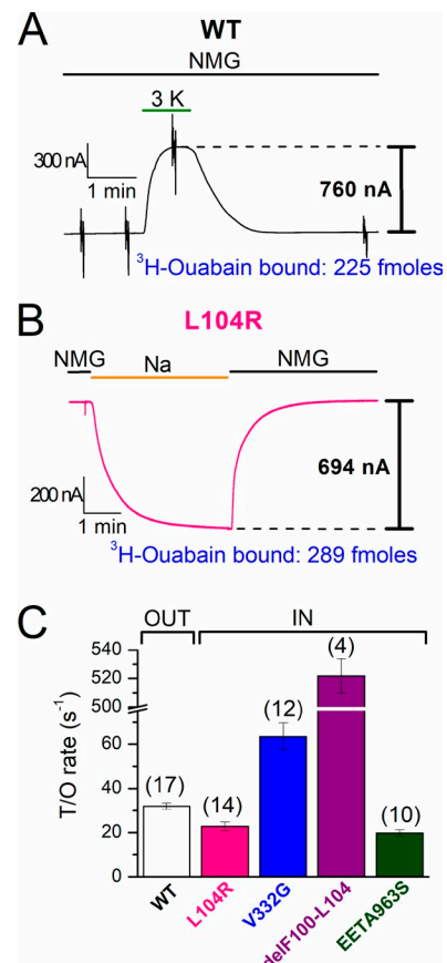
Figure 7. Turnover rates of wild-type and mutant human Na/K pumps. (A) Representative recording from an oocyte expressing wild-type pumps, held at -50 mV, in which application of 3 mM K + in NMG + induced outward current. (B) Representative recording from an oocyte expressing L104R pumps in which replacing NMG + with Na + solution induced inward current. The quantity of [ 3 H]ouabain bound to the oocytes in A and B is also indicated. (C) Bar graph showing mean turnover rates (moles of charge per second/moles of [ 3 H]ouabain bound; i.e., s -1 ) measured in individual oocytes, for the outward current (bracketed as “OUT”) in oocytes expressing wild type (n = 17) and for the Na + -induced inward current (bracketed as “IN”) in oocytes expressing L104R, V332G, delF100-L104, and EETA963S. Measurements were performed 4–5 d after injection, except for delF100-L104, which was performed 3 d after injection because of large currents. Note the break along the y axis. The number of experiments is indicated in parentheses. Error bars represent SEM.
