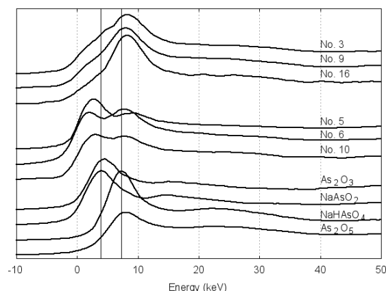
Figure 3: Arsenic speciation in hair samples of residents in an arseniasis hyper-endemic village. Left vertical line: Energy for As 3+ , right vertical line: Energy for As 5+ . As 2 O 5 , NaHAsO 4 : References for As 5+ ; NaAsO 2 , As 2 O 3 : Reference for As 3+ .
