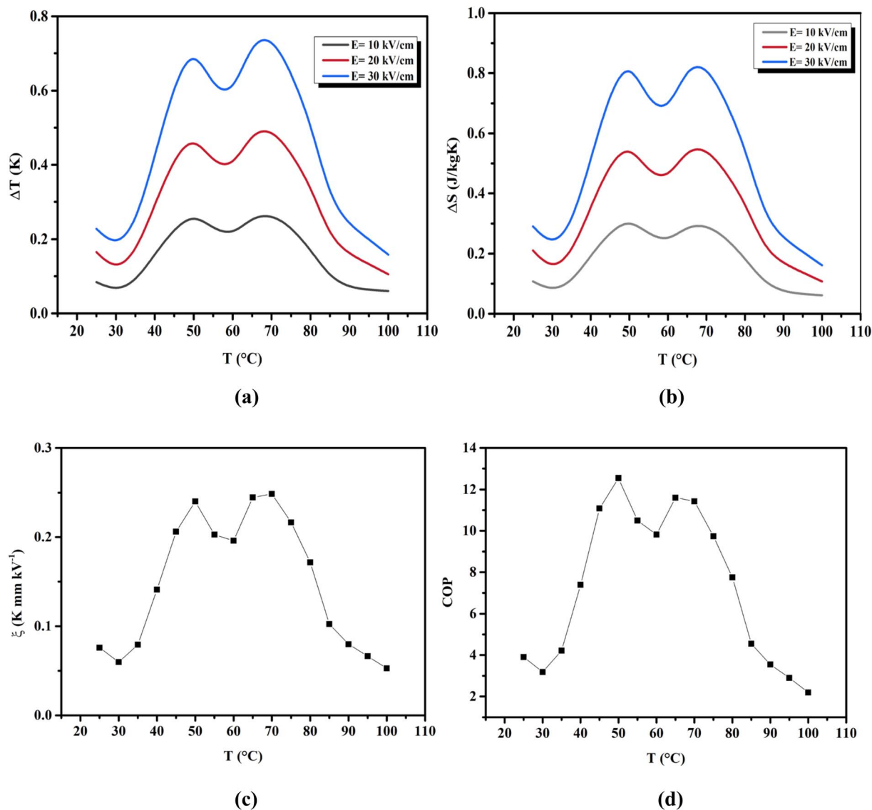
Fig. 8 Temperature dependence of (a) \Delta T , (b) \Delta S and (c) \xi for the BTSZ ceramic at different applied electric fields. (d) Temperature dependence of the COP.
