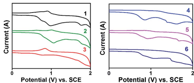
Fig. 2 Cyclic voltammogram of compounds 1–6.
