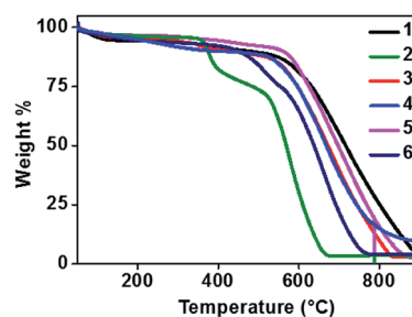
Fig. 3 TGA curves of compounds 1–6.
