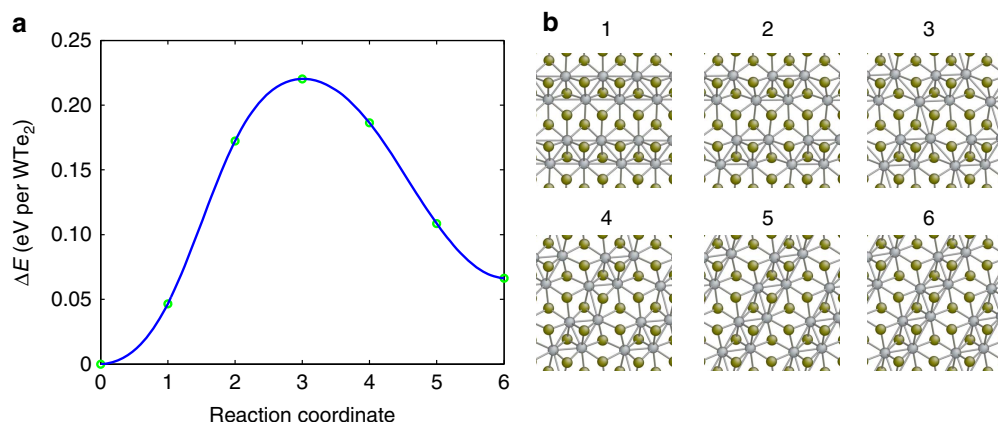
Figure 6 | NEB calculation of transformation barrier and the pathway for orientation switching. The initial configuration of the NEB calculation is the O1 variant of 1T'-WTe 2 monolayers at ground state (zero external stress), while the final state is the strained O2 variant with the same supercell dimensions as those of the O1 variant. (a) Change of the system energy per chemical formula unit as a function of reaction coordinate. (b) The corresponding atomistic structure of the system along the reaction coordinate. Four different supercells were used to carry out the NEB calculations: 2 \times 2 , 2 \times 4 , 4 \times 2 and 4 \times 4 supercell of the 1T' phase, which all give identical results.
