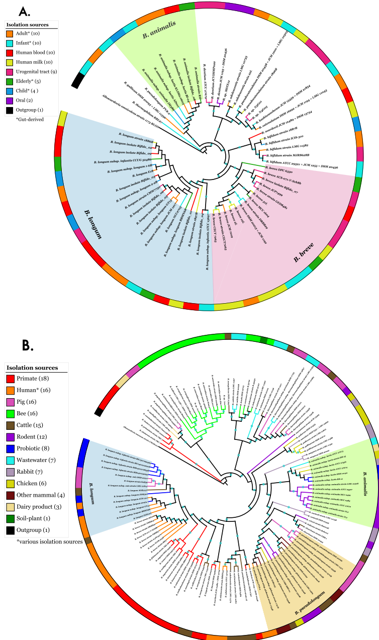
Fig. 1 Cladograms of bifidobacteria strains harbored by A) human hosts and B) multiple hosts and environments. 1A Phylogenetic relationship of human-derived Bifidobacterium strains based on 107 marker genes ( n = 60 + outgroup). The prominent species, B. longum (31.7%), B. breve (23.3%), and B. animalis (10%), are shaded in different colors. 1B Phylogenetic relationship of Bifidobacterium strains harbored by multiple hosts based on 107 marker genes ( n = 129 + outgroup). The prominent species, B. pseudolongum (12.4%), B. longum (10.9%) and B. animalis (10.1%), are shaded in different colors. For both cladograms, the outermost ring represents the different isolation sources. Bootstrap values higher than 70% are represented with blue circles. Strains from the Alloscardovia genus were used as outgroups for both phylogenetic trees (accession numbers JWA101000000 and NEKB01000000). Note that the “child” category refers to ages 2 through 6 years old while “infant” is younger. The “mammal” category indicates a mammal with only 1 sample size, including giraffe ( n = 1 ), hippopotamus ( n = 1 ), llama ( n = 1 ), and wallaby ( n = 1 ). Also, the “primate” category indicates non-human primates, and “probiotic” had an original, unknown isolation source that may overlap with the other categories
