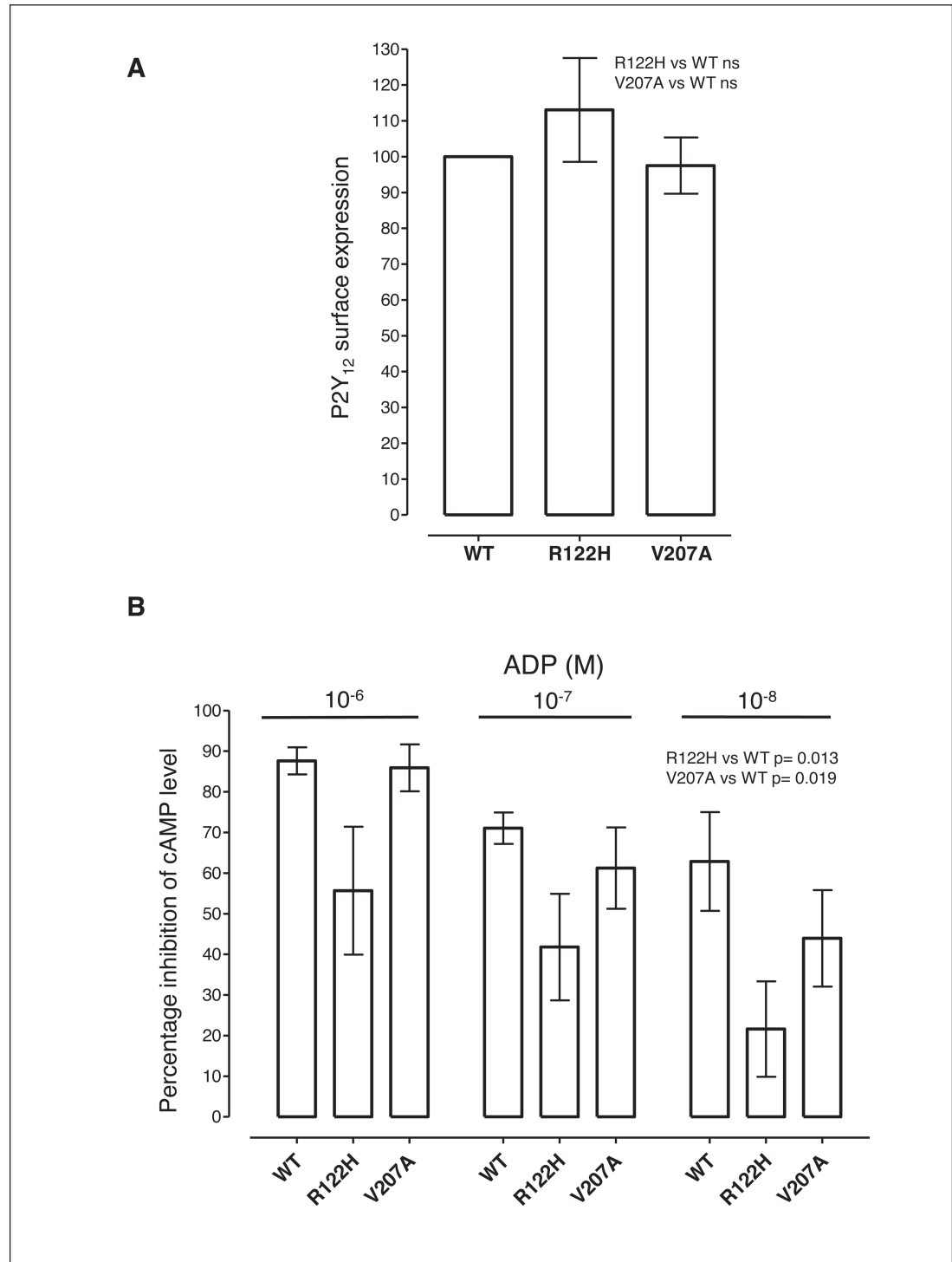
Figure 4: Cell surface expression and function of P2Y 12 R122H and V207A in transfected cells. A) Cell surface expression of HA-tagged P2Y 12 wild-type (WT), R122H and V207A was determined in transfected cells by ELISA using an anti-HA monoclonal antibody. Mean expression levels \pm SEM in three independent experiments are presented, normalised to expression of WT P2Y 12 . B) The ability of P2Y 12 WT, R122H and V207A to decrease cellular cAMP levels was determined in transfected cells by measuring residual cAMP by ELISA after incubation with the indicated concentrations of ADP. Data from three independent experiments are presented as the percentage inhibition (mean \pm S.E.M) of the basal cAMP level in forskolin-treated cells.
