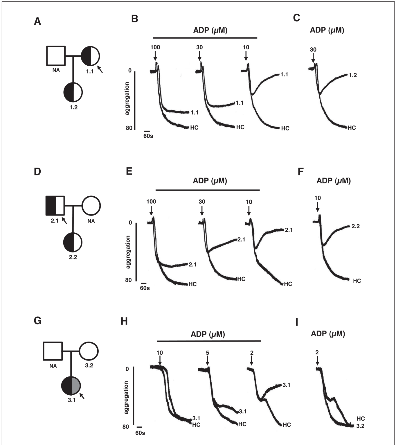
Figure 3: Platelet phenotype in cases with potentially damaging SNV in P2RY12. A) The pedigree of index case 1.1, who was heterozygous for the P2Y 12 R122H substitution (half back shading), showing pedigree member 1.2, also with the P2Y 12 R122H substitution. B) Light transmission aggregation (LTA) responses to 10–100 \mu M ADP in platelet-rich plasma from 1.1 and a healthy control (HC). C) LTA responses to 30 \mu M ADP in 1.2. D) The pedigree of index case 2.1, who was heterozygous for the P2Y 12 P258T substitution (half black shading) showing pedigree member 2.2, also with the
