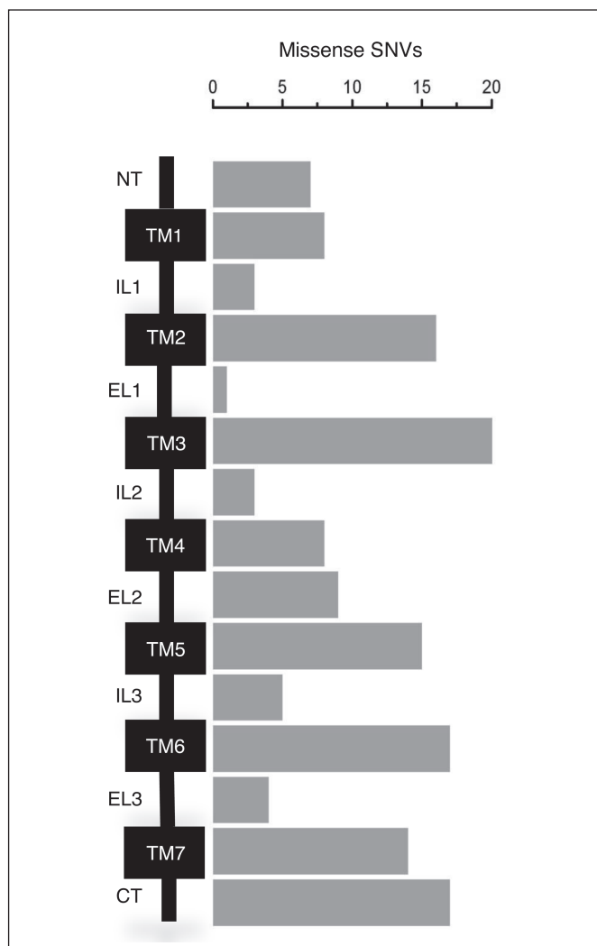
Figure 2: Distribution of potentially damaging missense SNVs across GPCR domains. Schematic of a prototypical Class A GPCR showing the N-terminal extracellular region (NT), the transmembrane helices (TM1–7), the intracellular (IL) and extracellular (EL) loops, and the C-terminal intracellular region (CT). The number of missense SNVs in the population databases classified as potentially damaging within these regions are represented in the bar chart.
