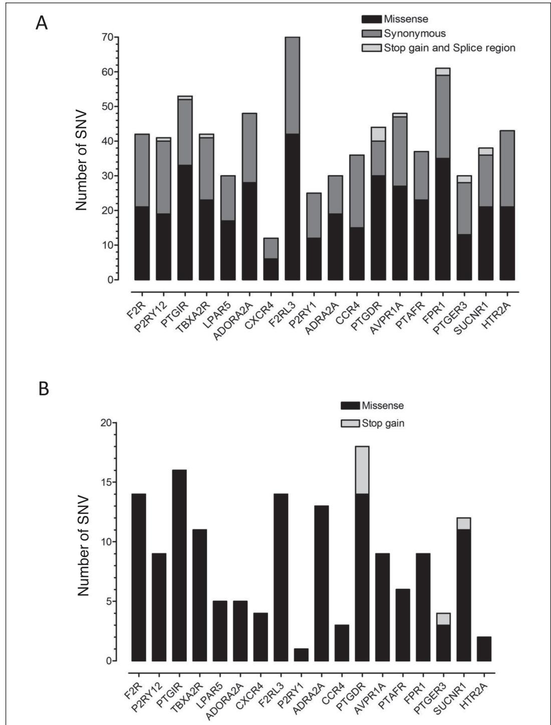
Figure 1: Distribution of SNVs in the target regions of 18 platelet GPCR genes in the ESP and 1,000 genomes datasets. A) The total number of unique SNVs in each GPCR gene found in the population datasets, subdivided according to whether missense, synonymous or stop-gain/splice region. B) The total number of unique SNVs in the population datasets that were classified as potentially damaging, subdivided according to whether missense or stop-gain.
