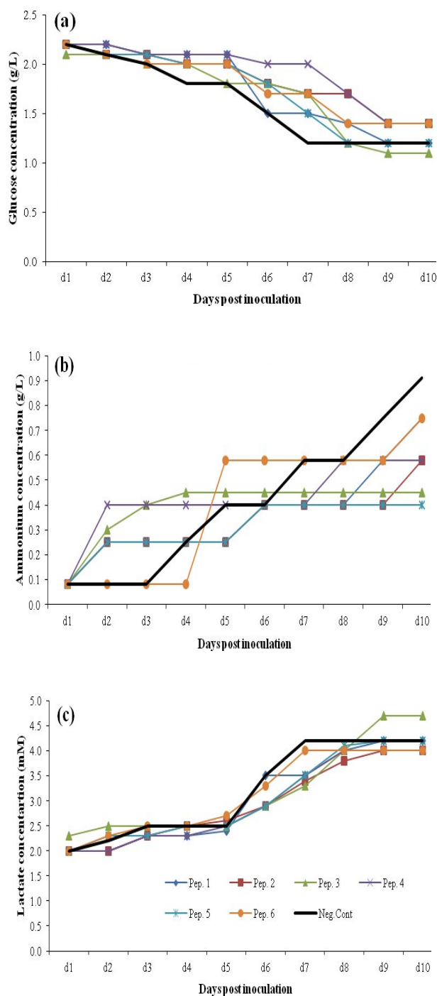
Fig. 8. Metabolic behavior changes in fed-batch cultures of the CHO cells using 1 \text{gl}^{-1} peptone (Pep) supplementations in CD DG44 medium. (a) Glucose concentrations, (b) ammonium concentrations, (c) lactate concentrations.
