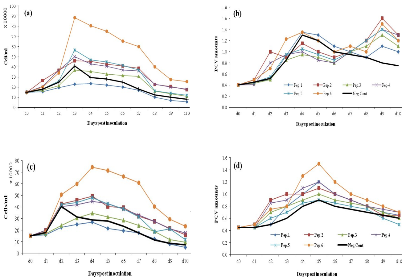
Fig. 3. The effect of 1 and 2 g -1 peptone (Pep) concentrations on cell density and PCV values of t-PA producing CHO DG44 cell line cultivated in ProCHO 5 medium. Viable cell numbers and PCV values in 1 g -1 (a and b) and 2 g -1 (c and d) peptone concentration.
