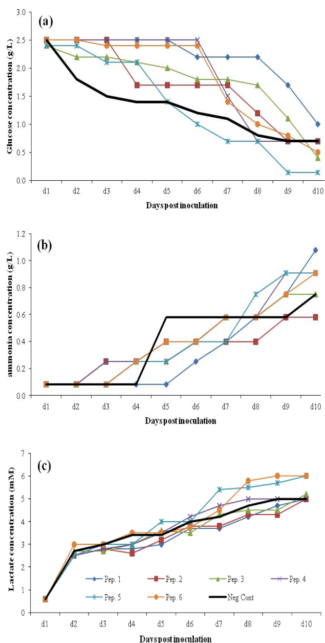
Fig. 7. Metabolic behavior changes in fed-batch cultures of the CHO cells using 2 \text{gl}^{-1} peptone (Pep) supplementations in ProCHO 5 medium. (a) Glucose concentrations, (b) ammonium concentrations, (c) lactate concentrations.
