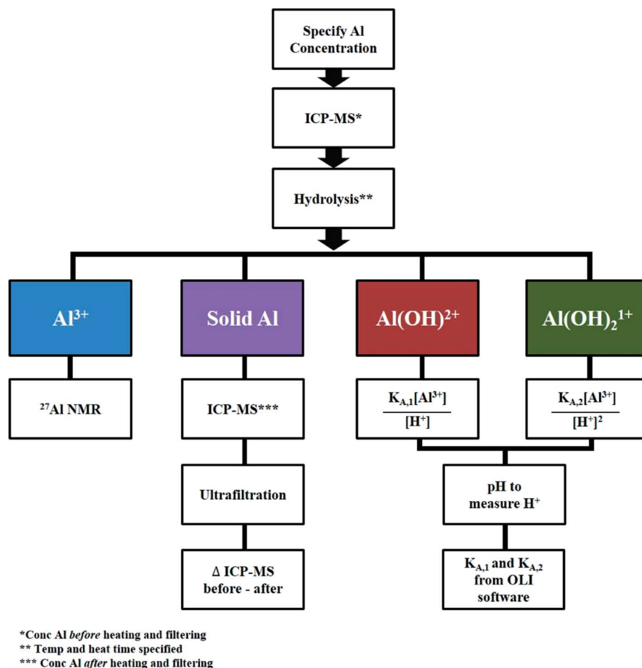
Fig. 4 Methodology to quantify aluminum speciation at specified concentrations of \text{AlCl}_3 and HCl, temperature, and heating time.
