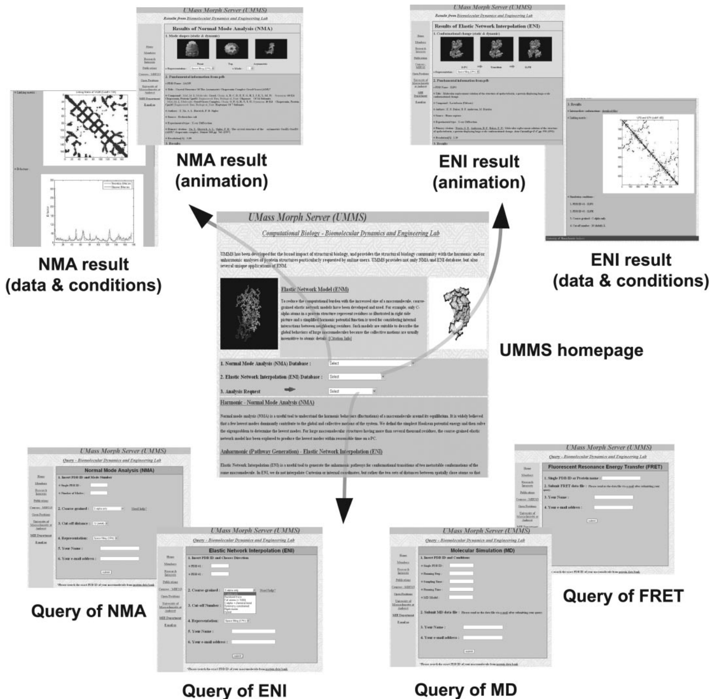
Figure 2. Overview of UMMS. The main page (middle panel) consists of NMA database, ENI database and query windows. One can not only browse NMA or ENI database to access the existing result of a specific macromolecule of interest, but also request the analysis via the query windows. A typical NMA window (upper left panels) shows animated mode shapes with various representations, the connectivity map of ENM called linking matrix, and the B-factor comparison plot. An ENI window (upper right panels) presents the computed ENI pathway between the two end conformations. One can download both animations and data files (PDB and text format) from those windows. Four different query windows (lower panels) are used for submitting the structural information of macromolecules (PDB ID, Cartesian coordinate file, MD trajectory data, FRET distance data) and choosing the simulation parameters (coarse-graining method, cutoff rule, output representation type).
