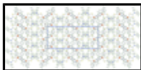
Fig. 2. A view in projection down the a axis of (I) showing the unit-cell contents. The C–H... \pi contacts are shown as purple dashed lines.
