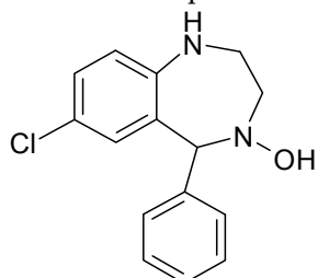
Demoxepam
