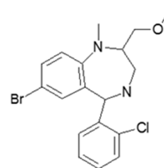
Metaclozepam
