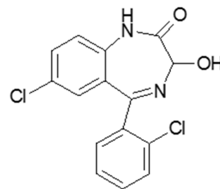
Lorazepam
