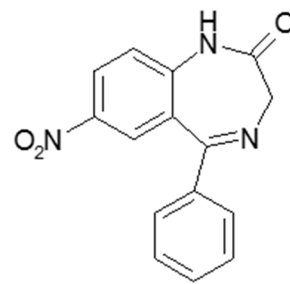
Nitrazepam
