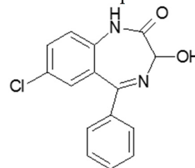
Oxazepam
