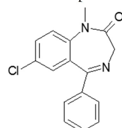
Diazepam
