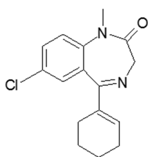
Tetrazepam
