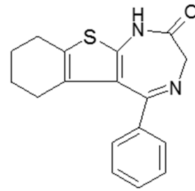
Bentazepam
