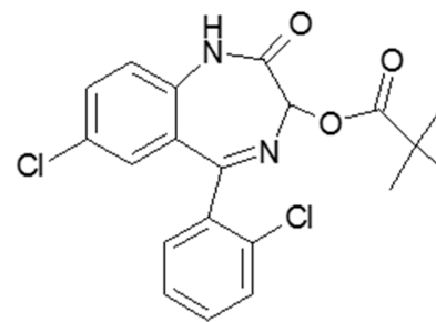
Pivazepam
