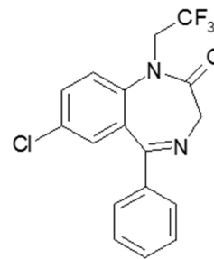
Halazepam
