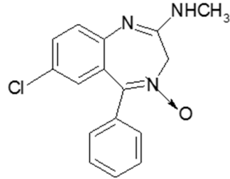
Chlordiazepoxide
