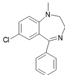
Medazepam
