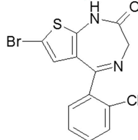
BrTDO
