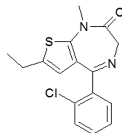
Clotiazepam
