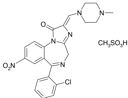
Loprazolam
