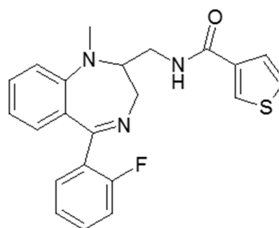
Tifluadom
