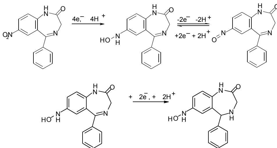
Scheme 1. Proposed voltammetric redox behavior of nitrazepam at a screen-printed carbon electrode.
