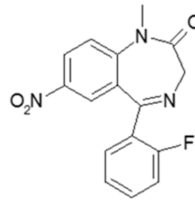
Flunitrazepam
