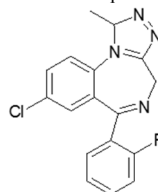
Midazolam
