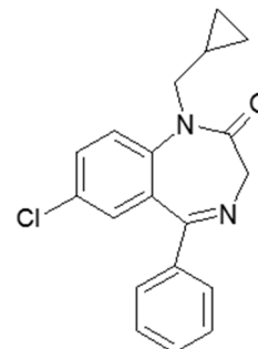
Prazepam
