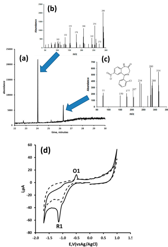
Figure 1. Gas chromatography of clonazepam and possible base hydrolysis product. (a) Full scan chromatogram; (b) hydrolysis mass spectrum (retention time 24.1 min); (c) clonazepam mass spectrum (retention time 26.2 min); and (d) cyclic voltammogram obtained in pH 11 phosphate buffer for a 1 mM clonazepam solution [116].
