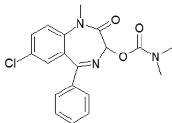
Camazepam
