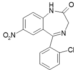
Clonazepam
