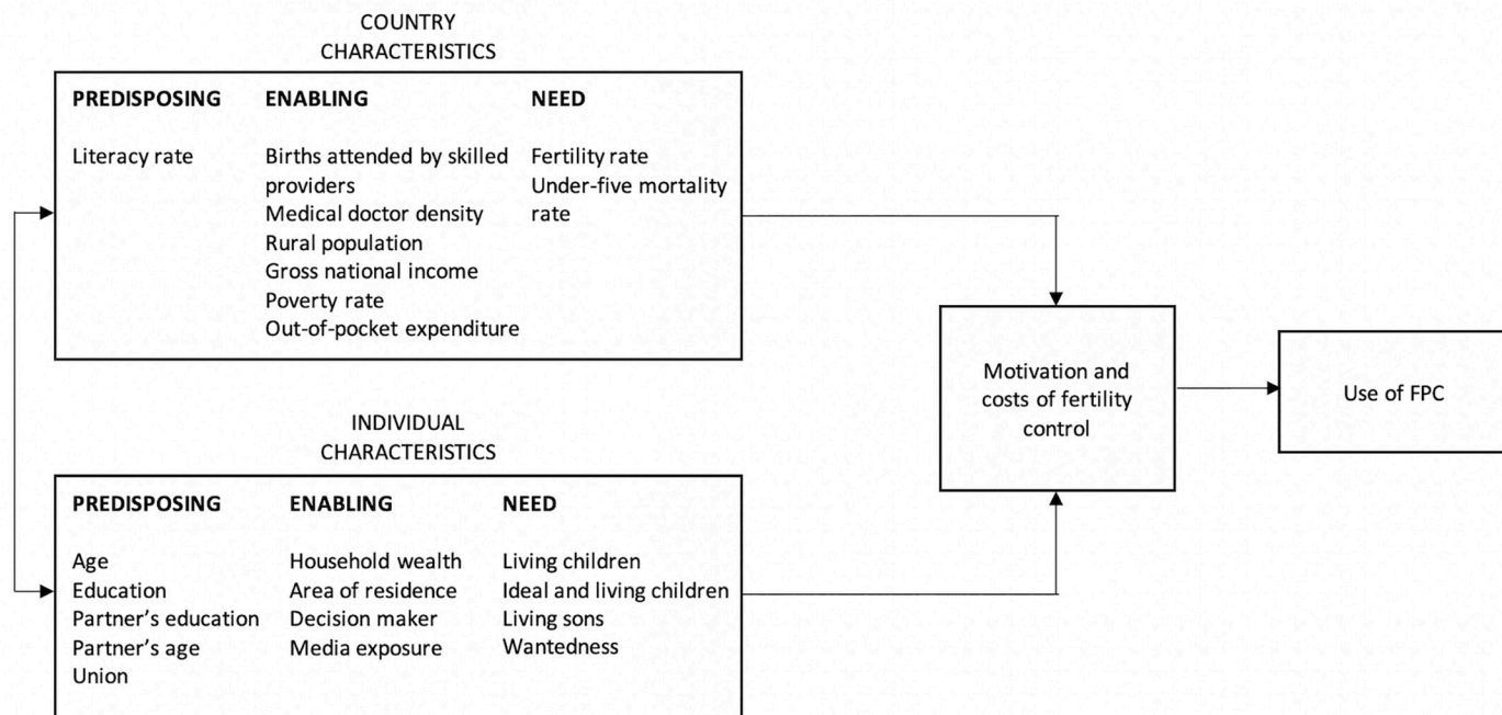
Fig 1. Conceptual framework.
