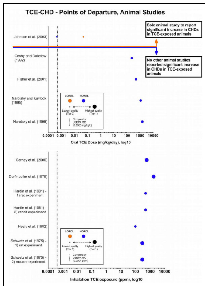
Figure 3. Summary diagram of exposure–response data for trichloroethylene (TCE) exposure via oral (A) or via an inhalation route (B) and congenital heart defects in experimental animal studies. Symbols represent intake dose as reported by original study authors. The color of the symbol indicates the type of effect: no observed adverse effect level (NOAEL; blue symbols) or the lowest observed adverse effect level (LOAEL; orange symbols). The size of the symbol indicates the overall risk of bias (ie, larger symbols indicate a lower risk of bias—or higher methodological quality, and vice versa). The dashed vertical line marks current United States Environmental Protection Agency (USEPA) reference concentration (RfC, A) and RfC (B).
