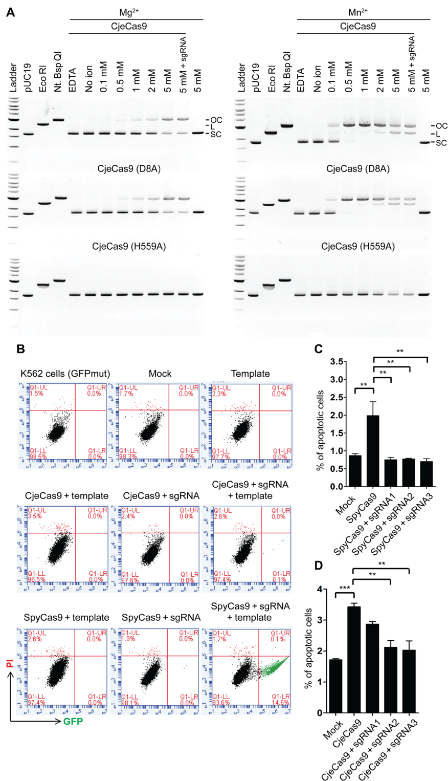
Fig. 4. In vitro cleavage assay and in vivo genome editing efficiencies of native CjeCas9 and SpyCas9 in human cells. (A) CjeCas9 activity and the effect of divalent cations ( Mn^{2+} and Mg^{2+} ) concentration on plasmid DNA cleavage. SC is super coiled, L is linear, and OC is open-circle plasmid DNA. (B) Restoration of GFP expression mediated by CjeCas9 or SpyCas9 genome editing in human cells [K562(GFPmut)] and quantified using FACS. In Q1-LR, the percentages of CjeCas9 or SpyCas9 genome edited cells that have a restored GFP expression are visualized (green). Q1-UL are dead cells. Q1-UR are GFP-positive dead cells. Q1-LL are unedited [K562(GFPmut)] cells. (C and D) Percentages of apoptotic human cells (K562) obtained after 6 hours. Concentration of CjeCas9 or SpyCas9 is 30 pmol, and for the sgRNA, the concentrations are 30, 60, and 90 pmol [for single guide RNA1 (sgRNA1), sgRNA2, and sgRNA3, respectively]. Results shown as means \pm SEM. *** P < 0.001 and ** P < 0.01 (one-way ANOVA, Bonferroni's multiple comparison test).
