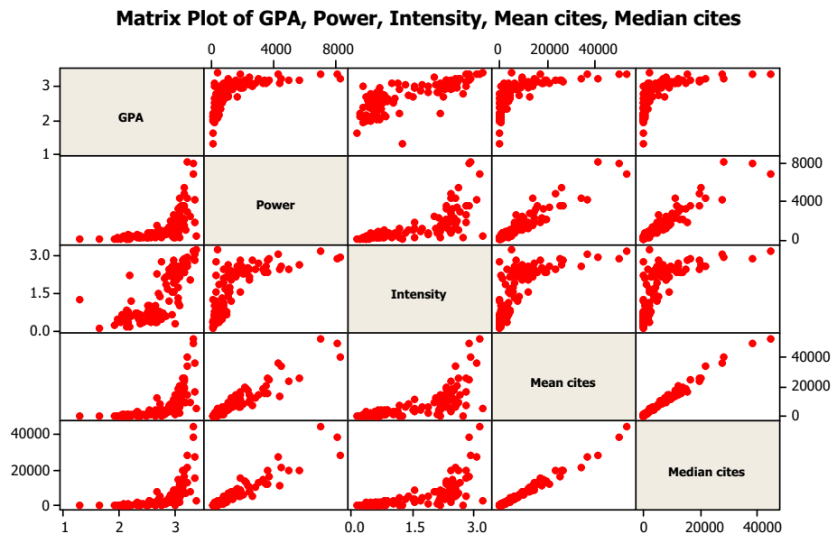
Fig. 1 Matrix plot of scattergrams for selected indicators
