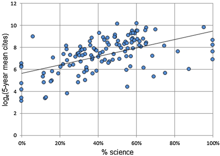
Fig. 4 Regression of \log_e(\text{mean 5-year cites}) against % science mix
