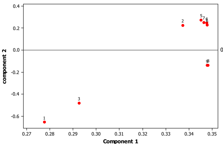
Fig. 2 First two principal components for the raw indicators. 1 GPA, 2 power, 3 intensity, 4 mean cites, 5 median cites, 6 mean 5-year cites, 7 median 5-year cites, 8 mean 5-year h -index, 9 median 5-year h -index
