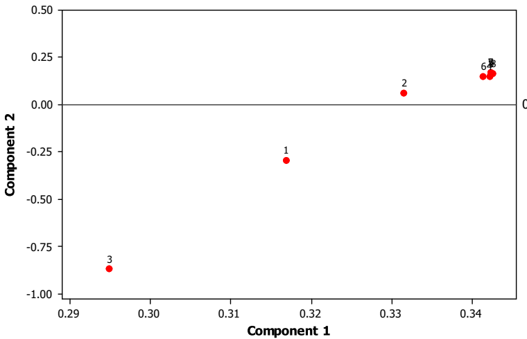
Fig. 3 First two principal components on ranked indicators. 1 GPA, 2 power, 3 intensity, 4 = mean cites, 5 median cites, 6 mean 5-year cites, 7 median 5-year cites, 8 mean 5-year h -index, 9 median 5-year h -index
