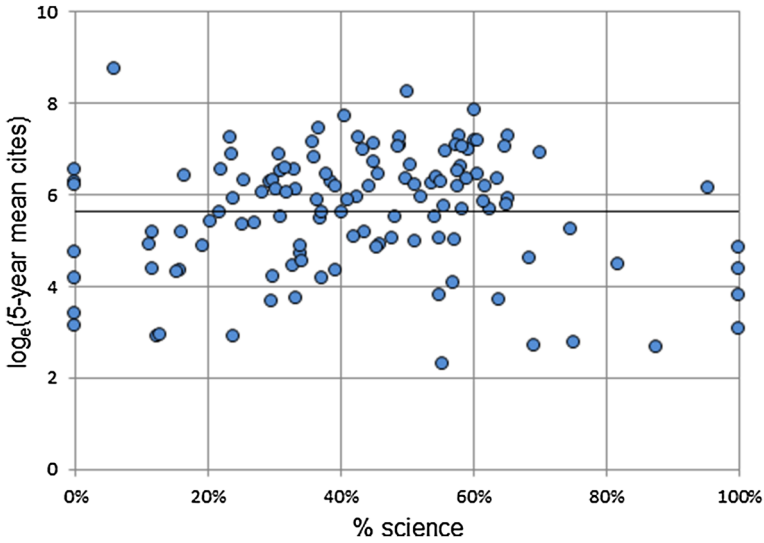
Fig. 5 Graph of log e (mean 5-year cites) adjusted for % science mix
