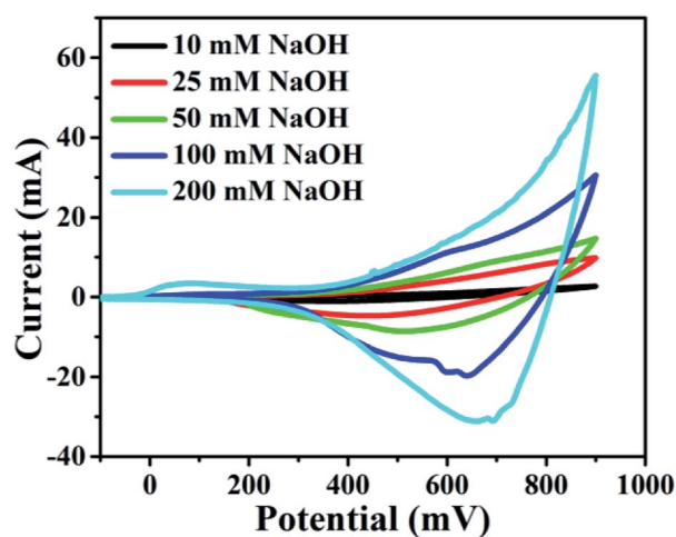
Fig. 7 Electrochemical effect of different concentrations of NaOH: 10 mM, 25 mM, 50 mM, 100 mM, and 200 mM with scan rate 100 \text{ mV s}^{-1} .
