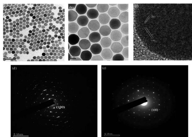
Fig. 2 TEM images of (a and b) NaYF 4 :Yb,Tm (88%/20%/2%) upconversion nanocrystals; (c) HRTEM image; SAED patterns of the (d) NaYF 4 :Yb,Tm (78%/20%/2%) upconversion nanocrystals and (e) NaYF 4 :Yb,Tm (88%/20%/2%) upconversion nanocrystals.
