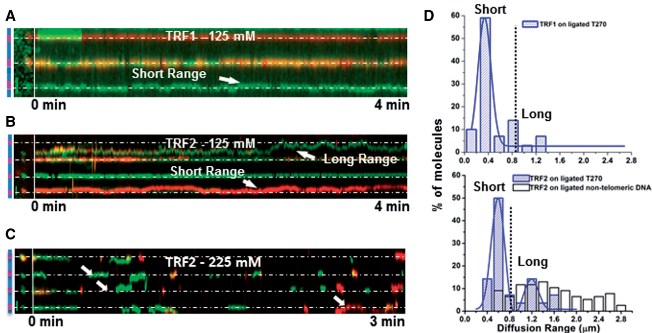
Figure 4. TRF1 and TRF2 show different diffusional properties over telomeric region versus nontelomeric regions. (A–C) Kymographical analysis of dual color (655 and 565 nm)-labeled TRF1 (A, 125 mM ionic strength) and TRF2 (B:125 and C:225 mM ionic strengths) on the ligated T270 DNA. The panel left to the vertical white line shows a schematic drawing of the ligated T270 substrate with telomeric (purple) and nontelomeric sequences (blue), and a fluorescence image of the DNA with protein-QDs. The horizontal white lines indicate the estimated center of the telomeric region based on the spacing between adjacent QDs. The white arrows in (C) indicate TRF2 diffusing between two adjacent telomeric sequences. (D) The diffusion range distributions of TRF1 (top, n = 29 ) and TRF2-QDs (bottom, n = 28 ) on the ligated T270 substrate (blue bars), and TRF2-QDs on the nontelomeric DNA (bottom, white bars, n = 77 ). Diffusion ranges below and beyond 850 nm are categorized into short (telomeric) and long range (nontelomeric), respectively. The lines in the top and bottom panels of (D) are single and double Gaussian fits to the data, respectively, which have R^2 of 0.90 and 0.96, respectively.
