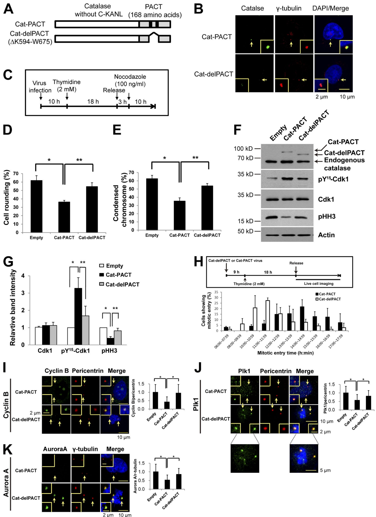
Figure 2. Effects of centrosome-targeted catalase on mitotic entry and on the abundance of centrosome-associated mitotic regulatory proteins. (A) Schematic representation of Cat-PACT (in which the centrosome-targeting PACT sequence replaces the C-terminal peroxisome-targeting sequence KANL of catalase) and Cat-delPACT (in which the sequence K594 to W675 of Cat-PACT containing two domains [black boxes] essential for centrosome targeting
