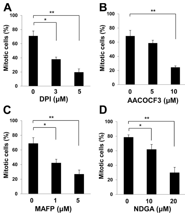
Figure 3. Sources of H 2 O 2 produced during mitotic entry. (A–D) HeLa cells stably expressing histone H2B–GFP were synchronized at G 1 –S by thymidine treatment for 18 h, released into S phase in thymidine-free medium for 3 h, and then incubated in medium containing nocodazole and various concentrations of DPI (A), AACOCF3 (B), MAFP (C), or NDGA (D) for 10 h. The percentage of mitotic cells was then estimated on the basis of chromosome condensation and cell rounding. Data are means ± SD from three independent experiments. *, P < 0.05; **, P < 0.005 (Student's t test).
