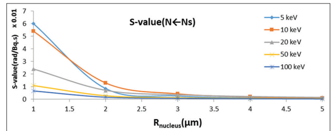
Figure 5: The absorbed dose per unit cumulated activity, S-value from nucleus surface to nucleus calculated for electrons with various energies (5–100 keV) for cell nucleus with radii of 1–5 \mu m
