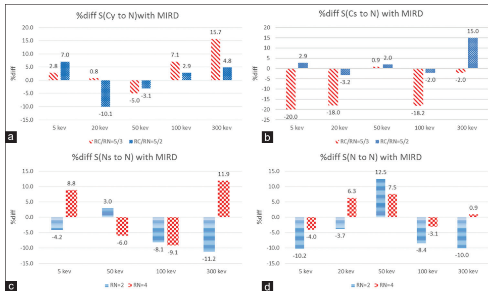
Figure 1: The S-value percentage difference between MIRD and Geant4-DNA data in this study in some selected geometries and compartments(a-d)
