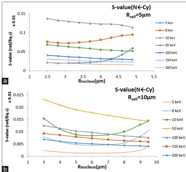
Figure 2: The absorbed dose per unit cumulated activity, S-value (N←Cy) calculated for electron with various energies (5–300 keV) for cells with (a) radius of 5 with nucleus radii 2.5, 2.8, 3.1, 3.4, 3.7, 4, 4.3, 4.6, 4.9 \mu m and (b) radius of 10 \mu m with nucleus radii 3, 4, 5, 6, 7, 8, 9, 9.5 \mu m
