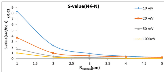
Figure 4: The absorbed dose per unit cumulated activity, S-value from nucleus to nucleus (N←N) calculated for electrons with various energies (10–100 keV) for cell nucleus with radii of 1–5 \mu m
