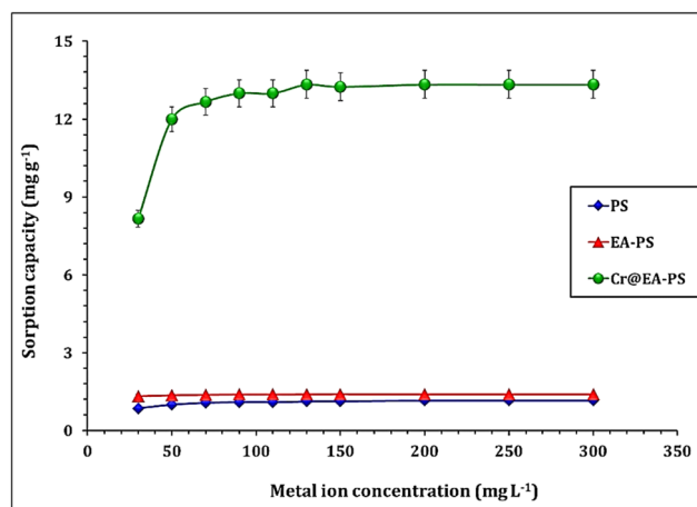
Fig. 9 Influence of metal ion initial concentration on the Cd(II) adsorption capacity (temperature of 25 ± 1 °C; pH 7.0; sorbent dosage of 3.0 g L; time is 240 min).
