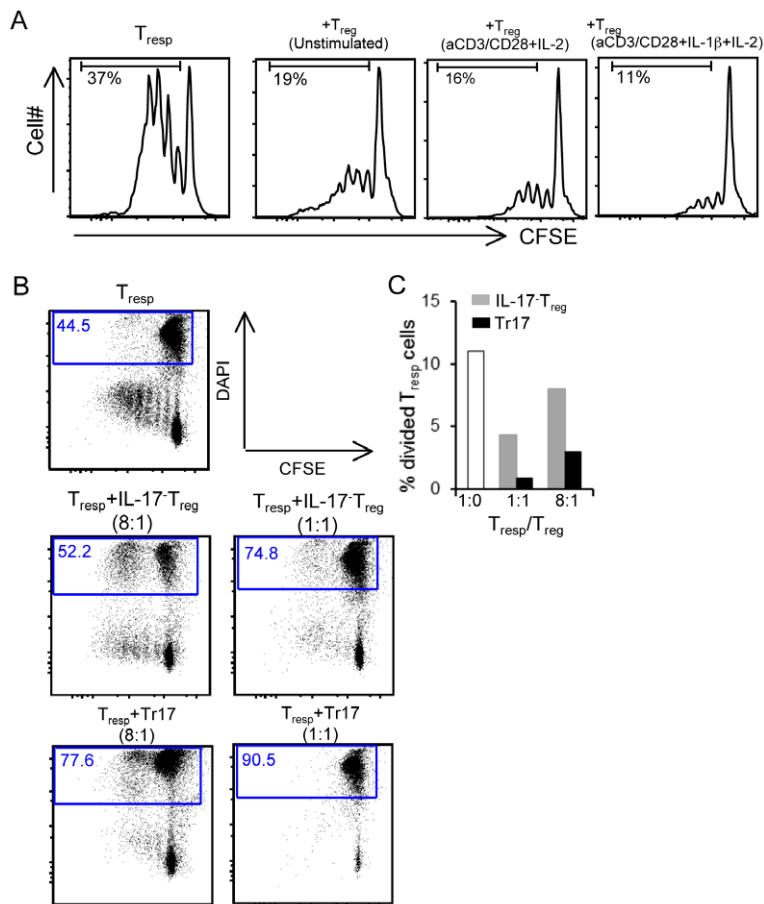
Figure 3. Tr17 cells display potent suppressive activity. (A) CFSE-labeled CD4^+CD25^- T cells (Tresp) from PL mice expressing Thy1.1 were cultured with anti-CD3/CD28 either alone or with indicated Tregs and cell divisions were assessed by CFSE dye dilution. The numbers indicate percent proliferating cells within total live Thy1.1 + cells (Tresp). (B) Tregs were cultured under polarizing conditions and IL-17 + and IL-17 - cells were sorted by cytokine capture and flow cytometry. CFSE-labeled Tresp cells from PL mice were cultured with anti-CD3/CD28 either alone or with Tr17 or IL-17 - Tregs for 4 d. Cell proliferation and death of Thy1.1 + Tresp cells were simultaneously assessed by co-staining with DAPI. Numbers indicate percent of dead cells within the Thy1.1 + population. (C) Proliferation of DAPI - Tresp cells was analyzed by flow cytometry. The data (A–C) are representative of three independent experiments. doi:10.1371/journal.pone.0045115.g003
