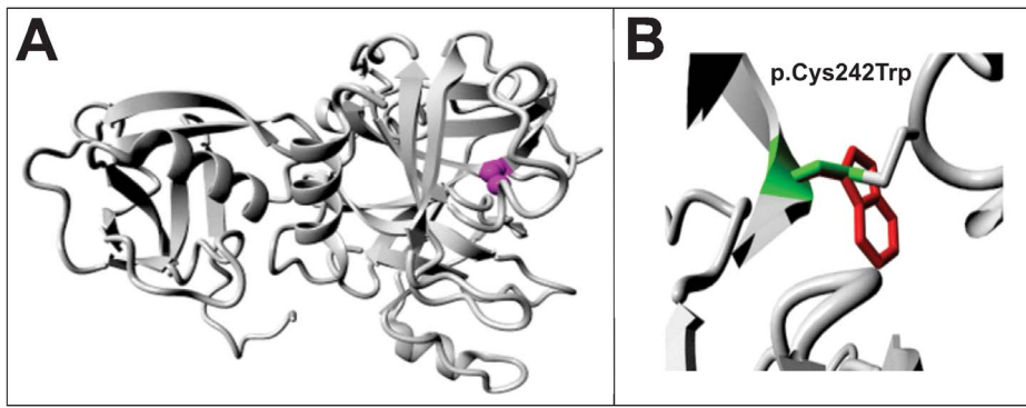
Figure 4. Predicted effect of mutation c.726C>G (p.Cys242Trp) on the three dimensional structure of TMPRSS3. A) Wild type protein structure with an intact disulphide bridge showing position of the mutated residue (magenta). B) Close-up view of the structure showing the wild type residue cysteine (green) and the mutant residue tryptophan (red). In case of the mutant residue there will be no disulphide bridge at this position.
