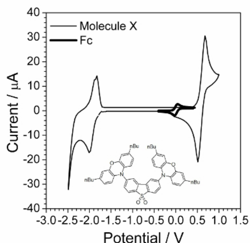
Figure 1: Cyclic voltammogram of investigated compound overlapped by cyclic voltammogram in presence of small amount of ferrocene. Solution: 1.0 \text{ mol} \cdot \text{L}^{-1} \text{Bu}_4\text{NBF}_4 and 0.01 \text{ mol} \cdot \text{L}^{-1} X in dichloromethane. Structure of compound X (2,8-bis(3,7-dibutyl-10H-phenoxazin-10-yl)dibenzo[b,d]thiophene-S,S-dioxide) is shown in the inset. Please click here to view a larger version of this figure.
