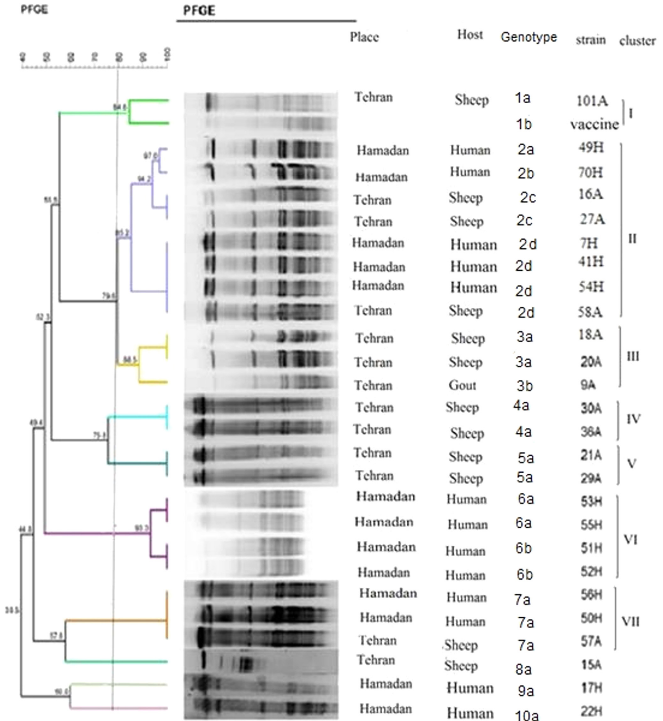
Fig. 4. PFGE dendrogram of human and animal Brucella isolates. A: animal; H: human.
