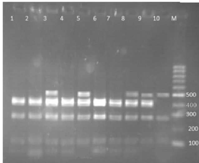
Fig. 2. Agarose gel electrophoresis of PstI restriction fragments of omp2a -PCR products. Lane 1, 2: human strains (Pattern 2), Lane 3: human strain (Pattern 1), lane 4, 6, 7 animal strains (Pattern 2), lane 5: Positive control ( B. melitensis biovar1 with Pattern 3), lane 8 animal strain (Pattern 1), lane 9 animal strain (Pattern 3), lane 10 animal strain (Pattern 4). Lane M: 100 bp molecular weight marker.
