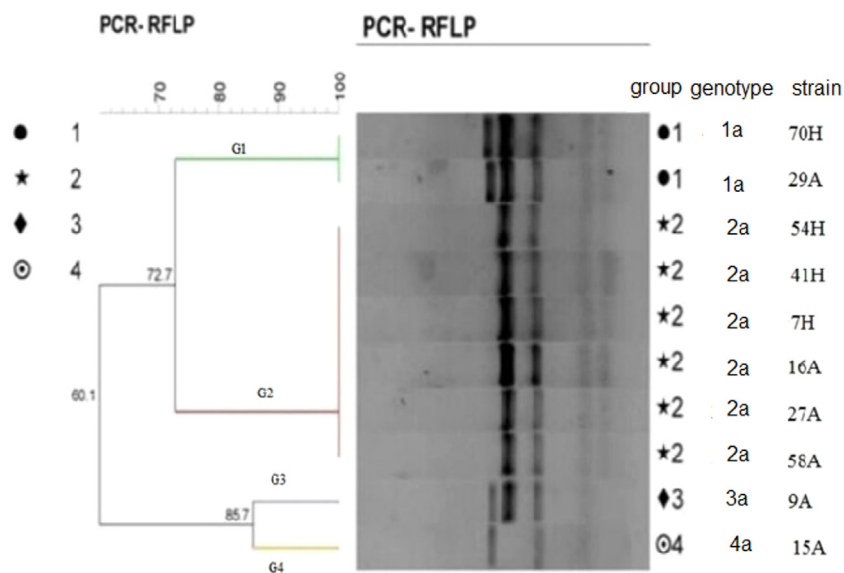
Fig. 3. PCR-RFLP dendrogram following pstI digested of omp2a gene amplification product. H: human, A: animal.
