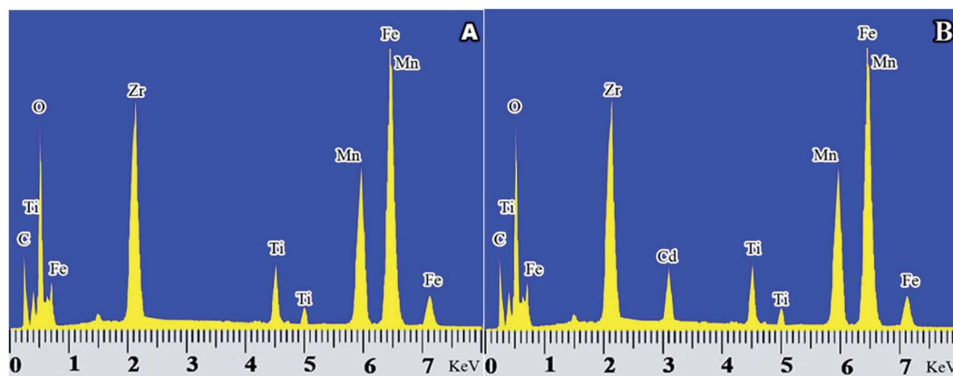
Fig. 12 EDX spectrum of the adsorbent sample synthesized before and after absorption of Cd(II), (A) of the EDX spectrum before adsorption of Cd(II), (B) of the EDX spectrum after adsorption of Cd(II).
