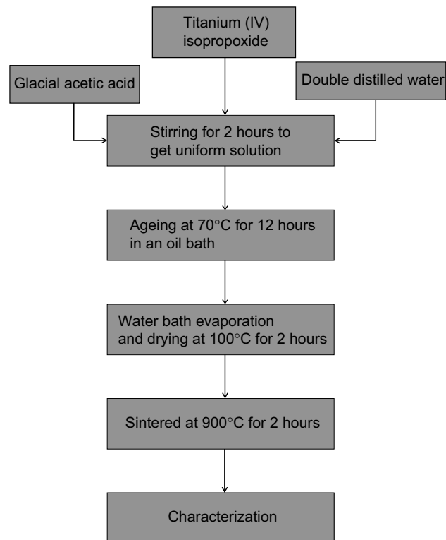
Figure 1 Flow chart for the synthesis of TiO 2 nanoparticles from Titanium (IV) isopropoxide via sol-gel process.
