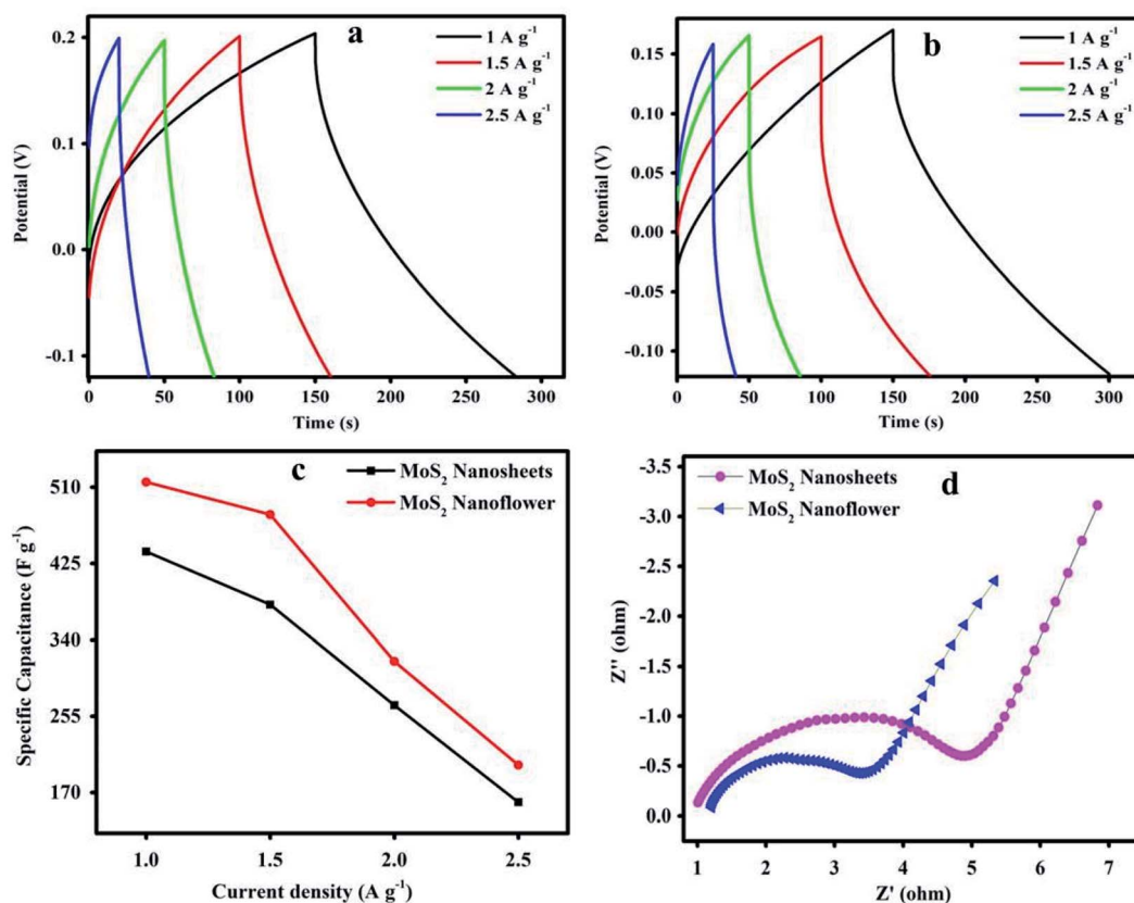
Fig. 7 GCD curve of the (a) MoS 2 nanosheets, (b) MoS 2 nanoflower, (c) MoS 2 nanosheets and MoS 2 nanoflower current density versus C_{\text{sp}} , and (d) Nyquist plot of the MoS 2 nanosheets and MoS 2 nanoflower.
