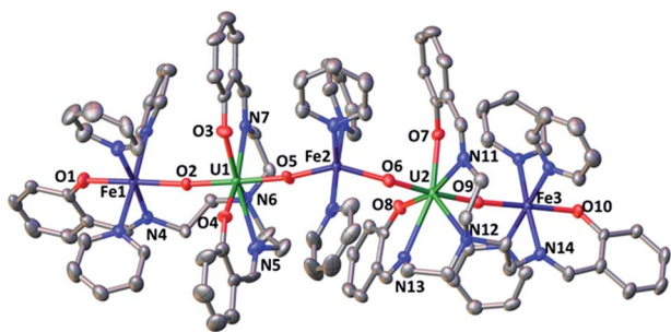
Fig. 6 Molecular structure of the dication [(\text{UO}_2(\text{trensal})\text{Fe}(\text{py})_3)_2\text{Fe}(\text{py})_3]^{2+} in 8 (H atoms were omitted for clarity, C atoms are represented in grey, O in red, Fe in dark blue, N in blue, U in purple and U in green). Selected distances U1–O2 = 1.920 (4) Å, U1–O5 = 1.935 (4) Å, U2–O6 = 1.927 (4) Å and U2–O9 = 1.927 (5) Å.
