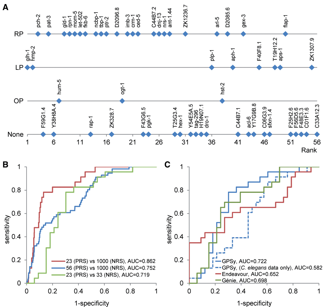
Figure 2. Gene ranking and RNAi phenotypes. (A) The most relevant phenotypes are plotted for each gene in the prioritized candidate list (from the 1st to the 56th, x -axis). On the y -axis, phenotype classes are indicated: RP = reproduction-associated phenotype; LP = lethal phenotype; OP = other phenotype; None = no observable phenotype. Official gene symbols are displayed for all genes. (B) Displays receiver operating characteristic (ROC) curves for: (i) the candidate gene set ( n = 56 genes) versus the C. elegans negative reference set (NRS; n = 1000 ; blue curve); (ii) the RP genes set ( n = 23 ) versus NRS (red); (iii) the RP versus non-RP sets (union of LP, OP and None phenotype; n = 33 ; green). The corresponding area under the ROC curve (AUC) values are indicated. Note the significant improvement in AUC value between (ii) and (i). The AUC value for (iii) is significantly non-random. (C) Displays ROC curves for the discrimination of the C. elegans RP ( n = 23 ) versus non-RP sets ( n = 33 ) using GPSy (default settings, solid blue line), GPSy ( C. elegans data only, dashed blue line), Endeavour (red) and Génie (green).
