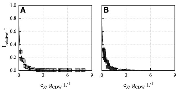
FIGURE 6 Relative photon flux densities ( I_{\text{relative}} ) in flat-panel gas-lift reactors as function of cell dry weight concentration c_X of D. salina CCAP 19/18. The parameter \epsilon (specific extinction coefficient) of the modified Lambert-Beer light attenuation model (—) was estimated both with the data of the batch processes with the “BG11+” (A, light grey) and “BG11 Biomass” medium (B, dark grey)
