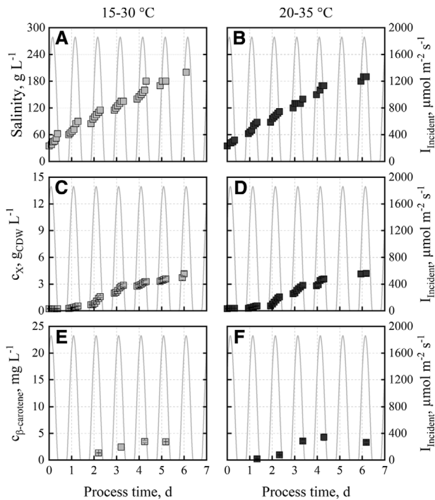
FIGURE 3 Salinities (A, B), cell dry weight concentrations (C, D) and \beta -carotene concentrations (E, F) during batch cultivations of D. salina CCAP19/18 with “BG11+” medium in flat-panel gas-lift photobioreactors operated at pH 8.5. The repetitively applied temperature profile of June 15, 2012 in Almería, Spain (15–30°C, light grey) was increased by 5°C to 20–35°C (dark grey) without changes in the day-night dynamics and the incident irradiance profile (0–1850 \mu\text{mol m}^{-2} \text{s}^{-1} ) of June 15, 2012 (Almería, Spain)
