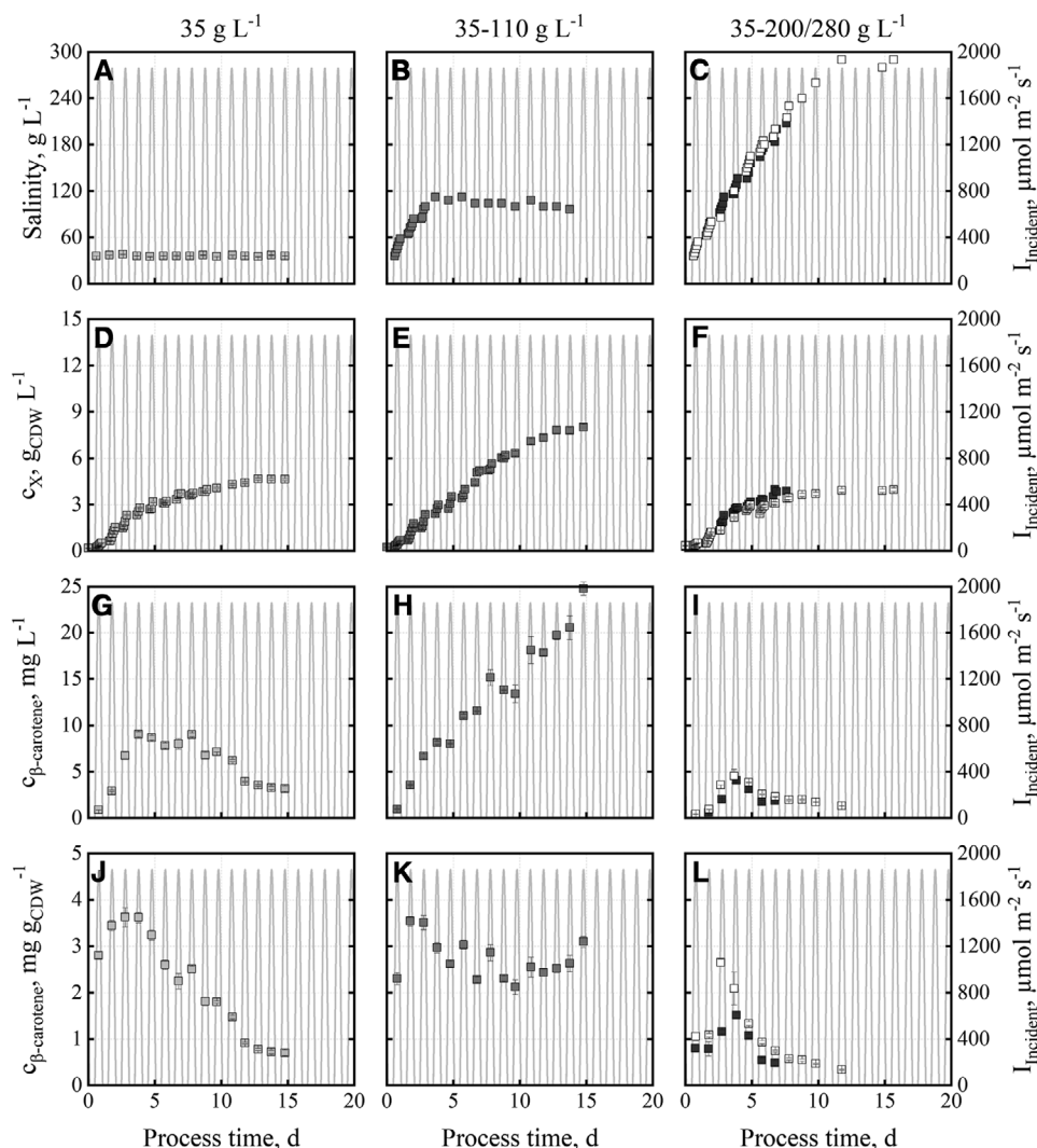
FIGURE 4 Salinities (A, B, C), cell dry weight concentrations (D, E, F), \beta -carotene concentrations (G, H, I) and \beta -carotene contents (J, K, L) during batch cultivations with D. salina CCAP19/18 in flat-panel gas-lift photobioreactors operated at pH 8.5 with “BG11+” medium. The salinity was constant at 35 \text{ g L}^{-1} (light grey), increased from 35 to 110 \text{ g L}^{-1} (grey) and increased from 35 to 200/280 \text{ g L}^{-1} (white, dark grey). Batch processes were carried out applying temperature ( 15\text{--}30^\circ\text{C} ) and incident irradiance profile data ( 0\text{--}1850 \mu\text{mol m}^{-2} \text{ s}^{-1} ) of June 15, 2012 in Almeria, Spain
