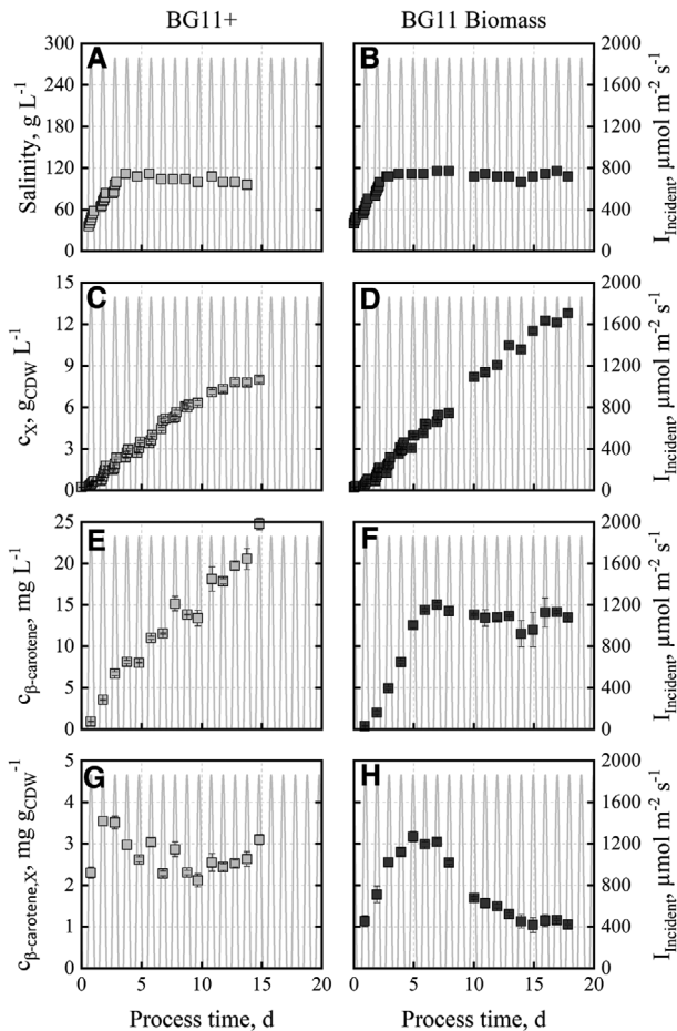
FIGURE 5 Salinities (A, B), cell dry weight concentrations (C, D), \beta -carotene concentrations (E, F) and \beta -carotene contents (G, H) during batch cultivations with D. salina CCAP19/18 at pH 8.5. The used media were “BG11+” (light grey) and “BG11 Biomass” (dark grey). The salinity was increased from 35 to 110 g L -1 . Batch processes were carried out at temperature (15–30°C) and incident irradiance profile data (0–1850 \mu\text{mol m}^{-2} \text{s}^{-1} ) of June 15, 2012 in Almería, Spain
