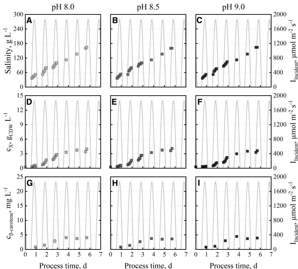
FIGURE 2 Salinities (A, B, C), cell dry weight concentrations (D, E, F) and \beta -carotene concentrations (G, H, I) during batch cultivations of D. salina CCAP19/18 with “BG11+” medium in flat-panel gas-lift photobioreactors operated at pH 8.0 (light grey), pH 8.5 (grey) and pH 9.0 (dark grey). Temperature (15–30°C) and incident irradiance profile data (0–1850 \mu\text{mol m}^{-2} \text{s}^{-1} ) of June 15, 2012 in Almería, Spain were applied repetitively
