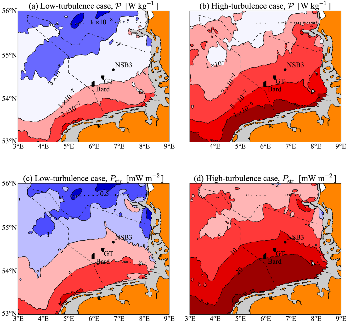
Fig 3. Map of estimated potential wind farm induced turbulence production in the German Bight region of the North Sea. Contours and colours show \mathcal{P} = P_{\text{str}}/(\rho_0 H) in units of \text{W kg}^{-1} (a, b) and P_{\text{str}} in \text{mW m}^{-2} (c, d). We have shown both low- and high-turbulence cases for the Bard 1 parameters with C_D = 0.35 in (a, c), and Global Tech 1 parameters with C_D = 1.0 in (b, d). The spatial pattern in (a, b) reflects the modelled distribution of \langle |\vec{u}|^3 \rangle , and the panels differ only by a factor of 4.6 (the difference in wind farm parameters for the high- and low-turbulence cases). The location of both the Bard 1 and Global Tech 1 (GT) farms are shown, along with the North Sea Buoy 3 (NSB3) measurement station. Grey areas are not included because they are on average less than 10 m deep, or comprise tidal flats or estuaries.
