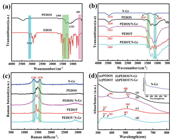
Fig. 1 (a) FT-IR spectrum of EDOS and PEDOS (b) FT-IR spectrum of N-Gr, PEDOS, PEDOS/N-Gr, PEDOT and PEDOT/N-Gr (c) Raman spectrum of N-Gr, PEDOS, PEDOS/N-Gr and PEDOT/N-Gr (d) UV-vis spectrum of N-Gr, PEDOS, PEDOS/N-Gr, PEDOT and PEDOT/N-Gr.
