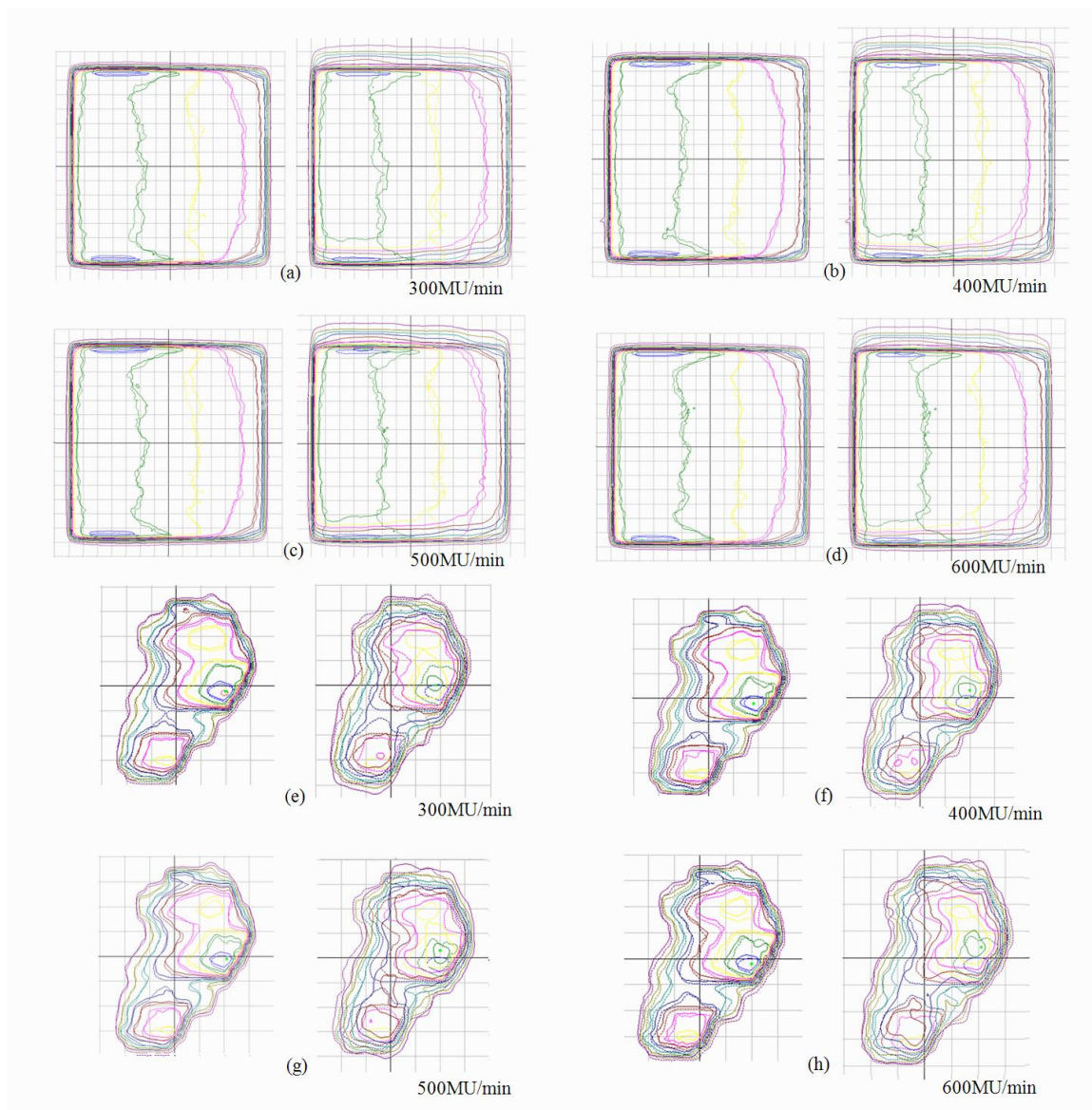
Figure 4 The dose distribution of film, comparing between static and moving target with gating (left) and without gating (right) for 30° wedge IMRT field (a-d) and lung IMRT plan (e-h). (Dashed lines for static and solid lines for moving target with and without gating)
