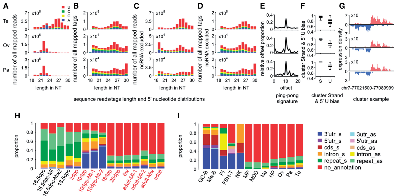
Figure 2. piRNA and piRNA features in mouse tissues. (A) Length distribution of all mapped sequence reads in three adult mouse tissues: Testes; Ov, ovary; Pa, pancreas. (B) Length distribution of all mapped sequence tags (sequence reads after collapsing identical sequences). (C and D) Length distributions of sequence reads and tags, excluding reads mapped to known ncRNA, respectively. Note that 5' uridine bias is one known property of primary piRNA. (E) Proportions of complementary small RNA reads (24–32 nt) at different offsets. Excess of complementary reads at offset equal 10 nt indicates the ping-pong model signature. (F) The stand (S) and the 5' uridine (U) bias of sequence reads' clusters based on 24–32 nt long sequences. (G) Reads coverage of a bidirectional piRNA cluster previously identified in mouse testes (4) in three mouse tissues. Shown are all reads with length 24–32 nt, excluding reads mapped to known ncRNA. The y-axis shows log 2 -transformed nucleotide coverage normalized by the total number of mapped reads within in a given sample. (H) Genomic context of piRNA clusters found in mouse testes at different age, from embryonic stages, pre-pachytene (10 dpp) and pachytene (18 dpp) stages to adults, based on data from (7,10,16,26,27) ('Materials and Methods' section). The labels indicate the age of the samples in days post-conception (dpc), days post-partum (dpp) or weeks (w) and piRNA origin: testes tissue (no label) or immunoprecipitations of Mili (MI), Miwi2 (Mw2) or Miwi (Mw) proteins. For a full sample description, see Supplementary Table S13. (I) Genomic context of piRNA clusters in adult mouse tissues: GC-B, germinal center B cells; Ma-B, mature B cells; PI, plasma cells; FH-T, follicular helper T cells; NK, natural killer cells; MP, macrophages; MDD, macrophages-derived dendritic cells; Ne, neutrophils; HP, hematoopoietic progenitor cells; Ov, ovaries; Pa, pancreas; Te, testes (28).
