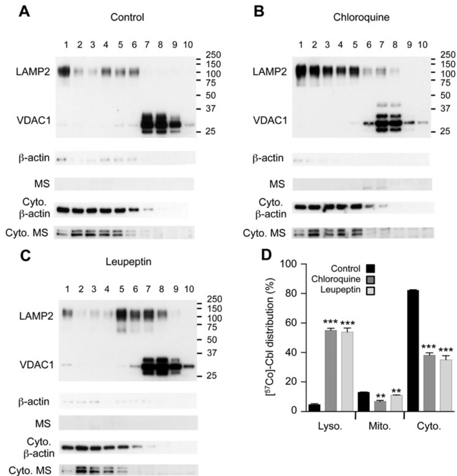
Figure 2 Protease inhibitors increase [ ^{57}\text{Co} ]Cbl retention in neuronal lysosomes
