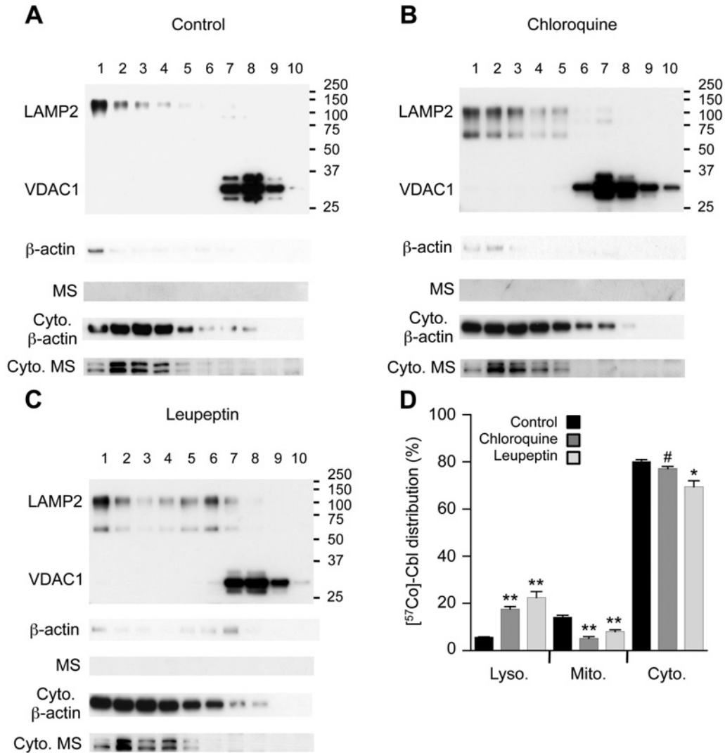
Figure 1 Protease inhibitors increase [^{57}\text{Co}]\text{Cbl} retention in fibroblast lysosomes Approximately 16 \times 10^6 HT1080 fibroblasts were metabolically labelled with [^{57}\text{Co}]\text{Cbl} for 48 h. The radiolabelled cells were disrupted using a ball-bearing homogenizer and the lysosomal, mitochondrial and cytosolic fractions were separated using an OptiPrep gradient. Intracellular marker proteins LAMP2 (lysosomal), VDAC1 (mitochondrial), \beta -actin and MS (cytosolic) were then probed by Western blotting in all fractions. Cells were assessed under the standard 'Control' culture conditions (A) and after the treatment with 25 \mu\text{M} chloroquine for 48 h (B), 40 \mu\text{M} leupeptin for 48 h (C). The proportional distribution of [^{57}\text{Co}]\text{Cbl} was assessed using a gamma counter and expressed as a percentage of radioactivity in each fraction (D). Positions of molecular mass markers (kDa) are shown on the blots. Fractions are labelled 1–10, from lightest (top of gradient) to heaviest (bottom of gradient). Cyto, cytosol. (A–C) Data are representatives of three independent experiments. (D) Data are means with S.E. represented by the error bars ( n = 3 experiments for each condition). * P < 0.05 , ** P < 0.01 , # P = 0.07 .
