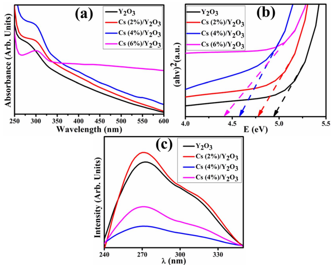
Fig. 4 (a) Absorption spectra, (b) band gap energy, and (c) emission spectra of Y 2 O 3 and Cs (2, 4, and 6 wt%) doped Y 2 O 3 NSs.
