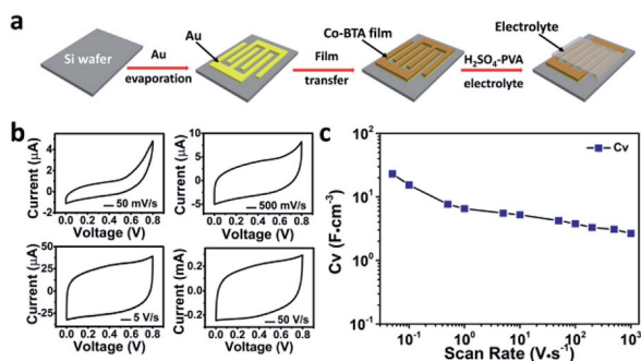
Fig. 4 (a) Schematic illustration of the fabrication of MSC device with the Co-BTA film electrode. (b) CV curves of Co-BTA-based MSCs in the H 2 SO 4 -PVA gel electrolyte at different scan rates. (c) C v evolution of the MSCs at different scan rates.
