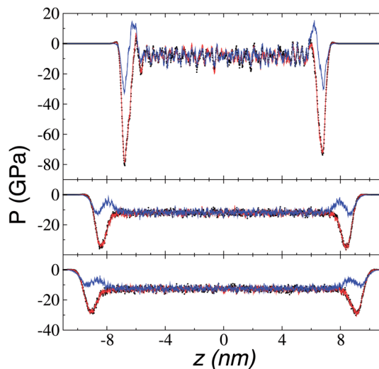
Fig. 10 Normal (blue) and transverse (red and black) pressure profiles as a function of position in the normal direction to the vacuum–liquid interface for [BMIM + ][BF 4 - ] ionic liquid at 373.15 K (top), 673.15 K (middle), and 773.15 K (bottom).
