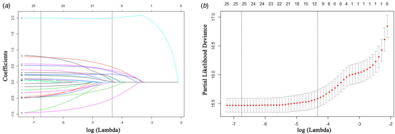
Fig. 2. Predictor selection using the least absolute shrinkage and selection operator (LASSO). (a) LASSO coefficient profile plot of 26 features for survival. Parameter (lambda) selection in the LASSO model adopted 10-fold cross-validation by the minimum criteria for survival.
