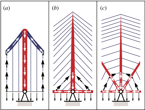
Figure 11. Appraising the relative efficiency of bridge forms by considering how deck loads are transmitted back to a support. (a) Suspension bridge: the load path is comparatively long, so a large volume of material is required to transmit the forces involved. (The same situation occurs in a fan cable-stayed bridge.) (b) Harp cable-stayed bridge: the load path is kept short, but acute angles between the elements lead to high cable forces, and also to significant induced forces in the deck. (c) Split-pylon cable-stayed bridge: the load path remains relatively short but the angles between the elements are less acute, ensuring cable and induced deck forces are lower. (Online version in colour.)
