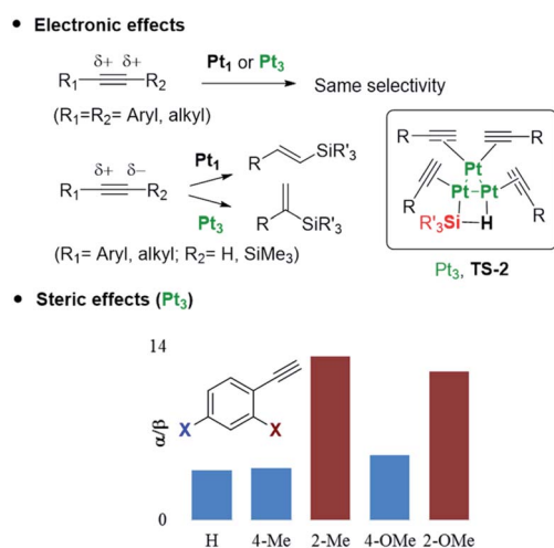
Fig. 6 Proposed transition state TS-2 during the hydrosilylation of alkynes with the Pt 3 catalyst, and electronic and steric factors of the alkyne affecting reaction regioselectivity for Pt 3 .
