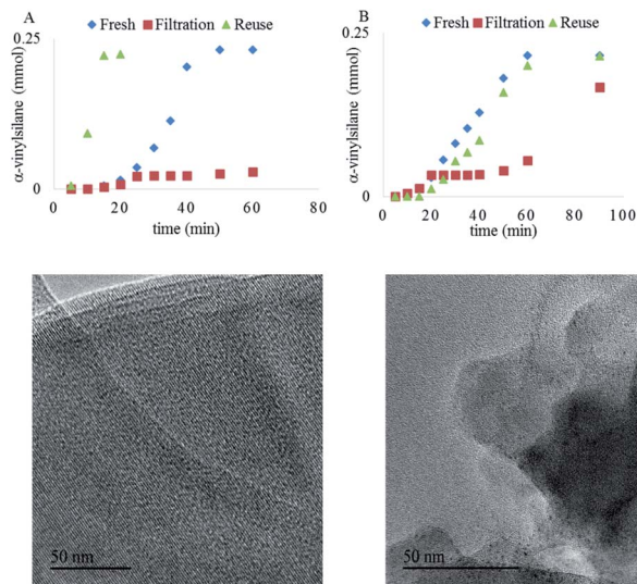
Fig. 9 Top: Hydrosilylation of 1-octyne 3 (0.5 M) with triethylsilane 2 (1.2 equivalents) in toluene (1 ml) at 110 °C using Pt_1/NaY (A) and Pt_3/NaY (B) as catalysts ( 2.5 \times 10^{-4} M). Bottom: High resolution transmission electron microscopy (HR-TEM) images of the Pt_1/NaY catalyst (A) fresh and (B) reused 5 times.
